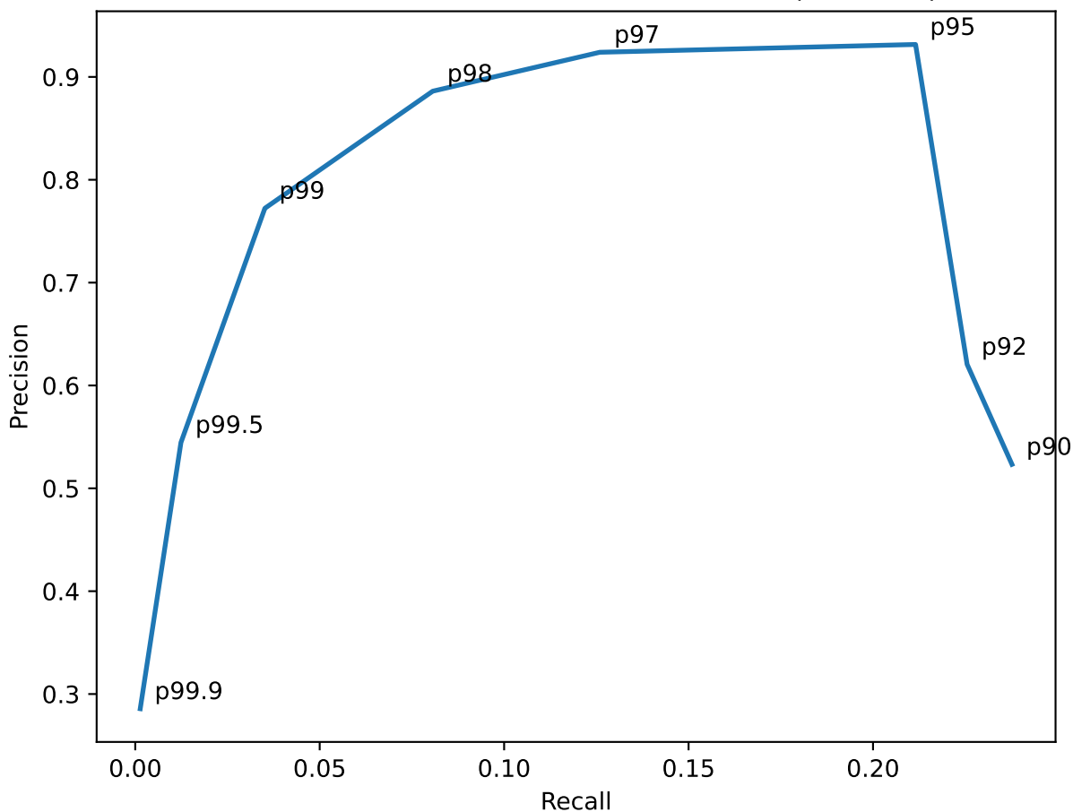
Matrix Profile: Precision-Recall trade-off (m=1440)
