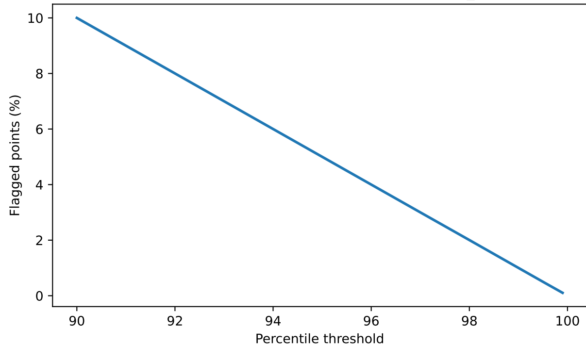
Rolling Z-score: Alarm rate vs percentile threshold (z_window=360)
