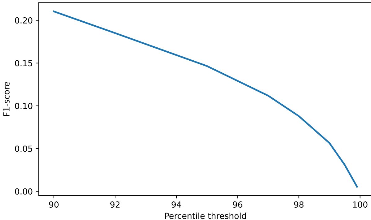
Rolling Z-score: F1-score vs percentile threshold (z_window=360)
