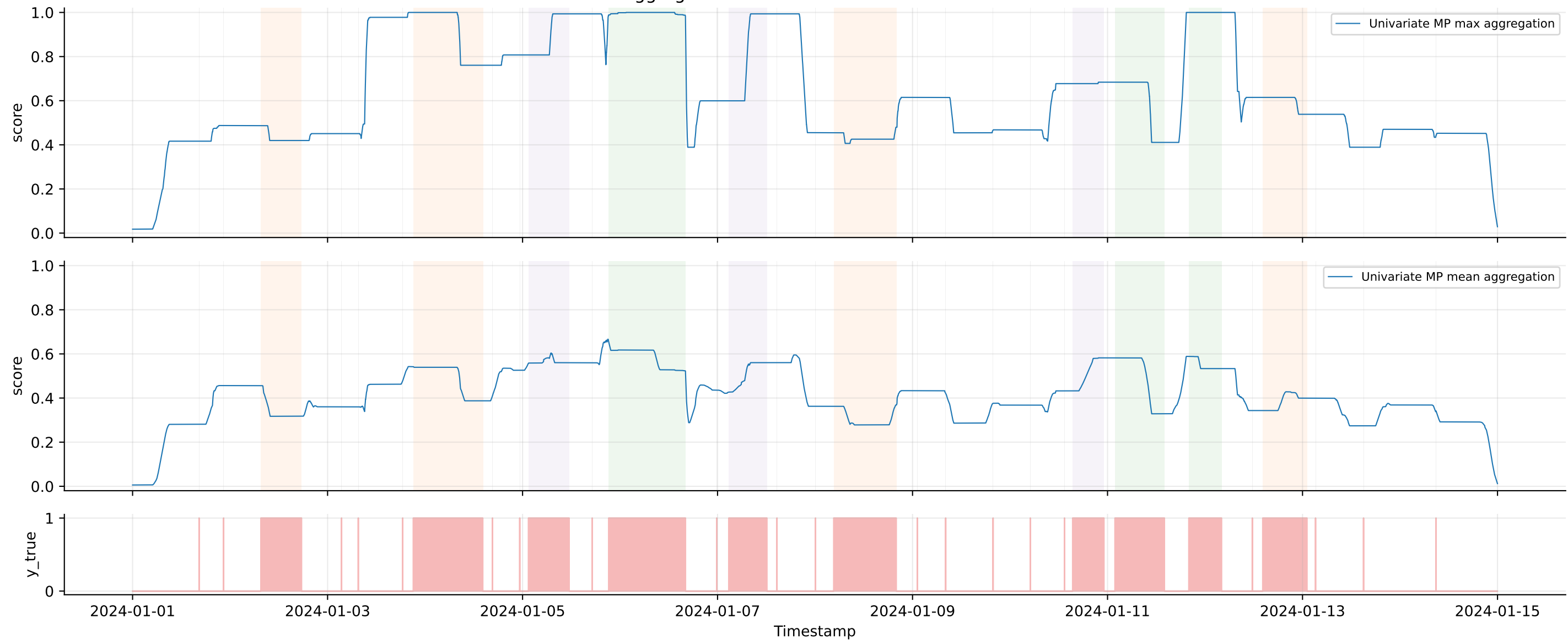
Aggregated Univariate Matrix Profile Scores
