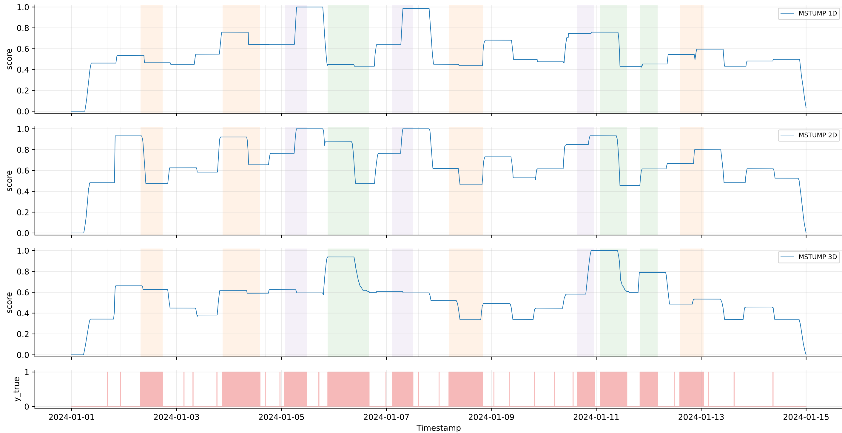
MSTUMP Multidimensional Matrix Profile Scores
