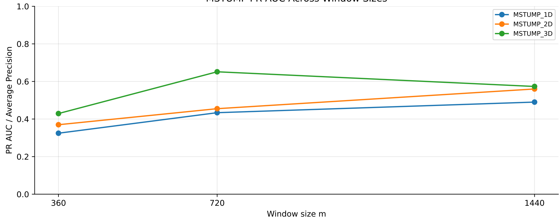
MSTUMP PR AUC Across Window Sizes
