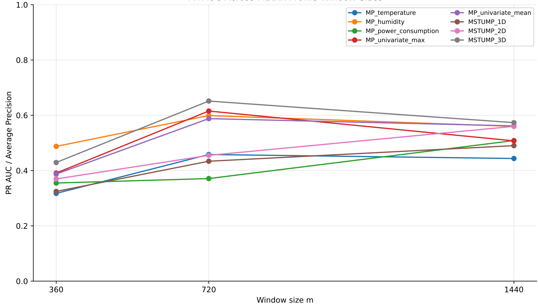
PR AUC Across Matrix Profile Window Sizes
