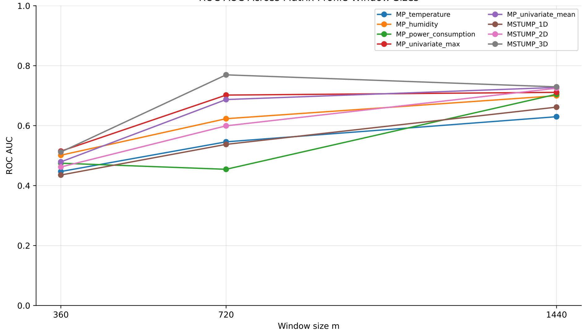
ROC AUC Across Matrix Profile Window Sizes
