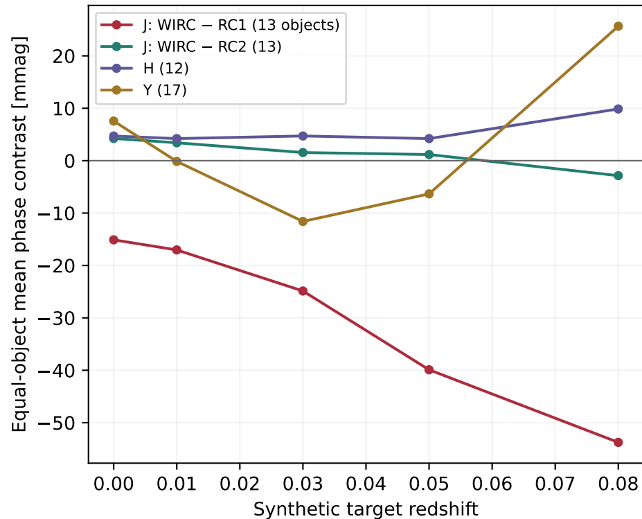
Same delivered spectral shapes, redshifted
