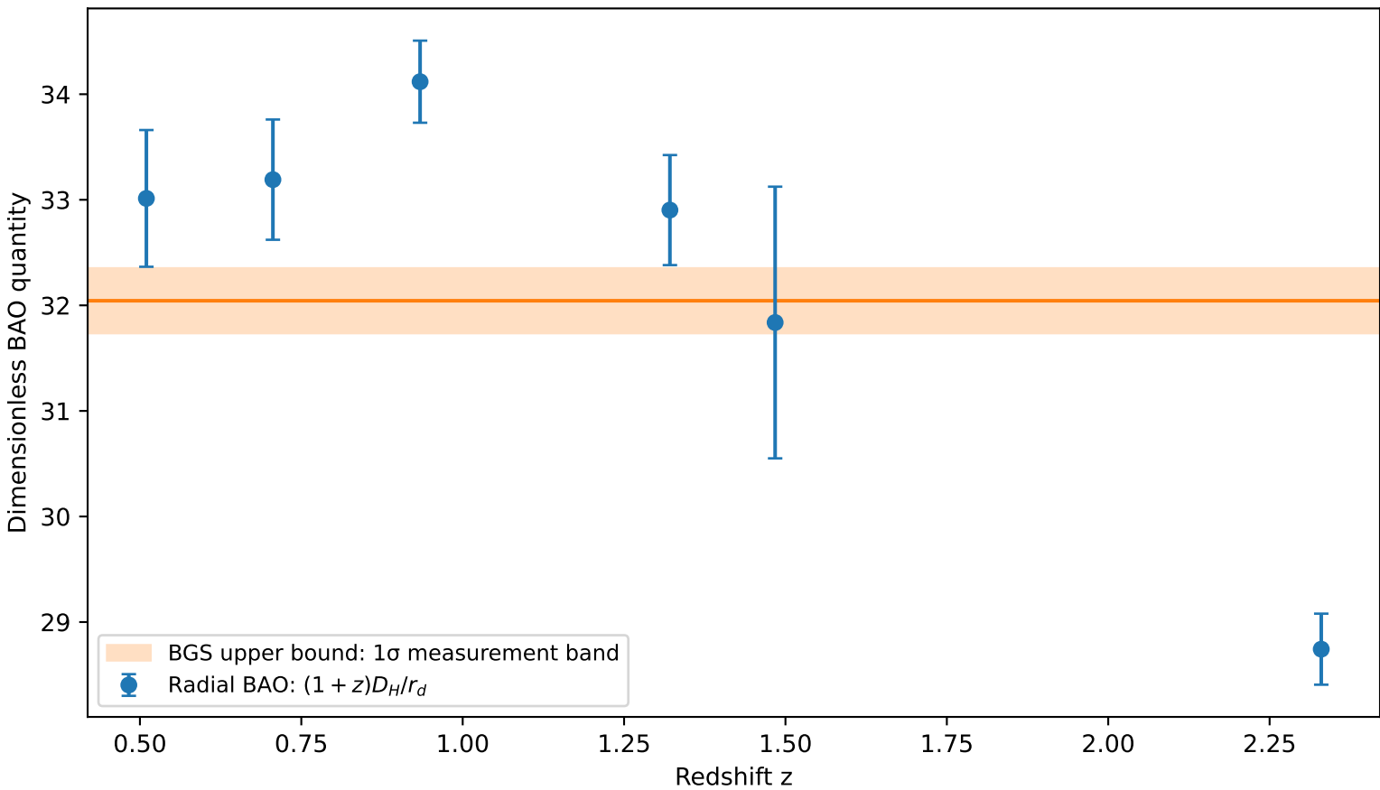
No acceleration + flat geometry requires every blue mean below orange
