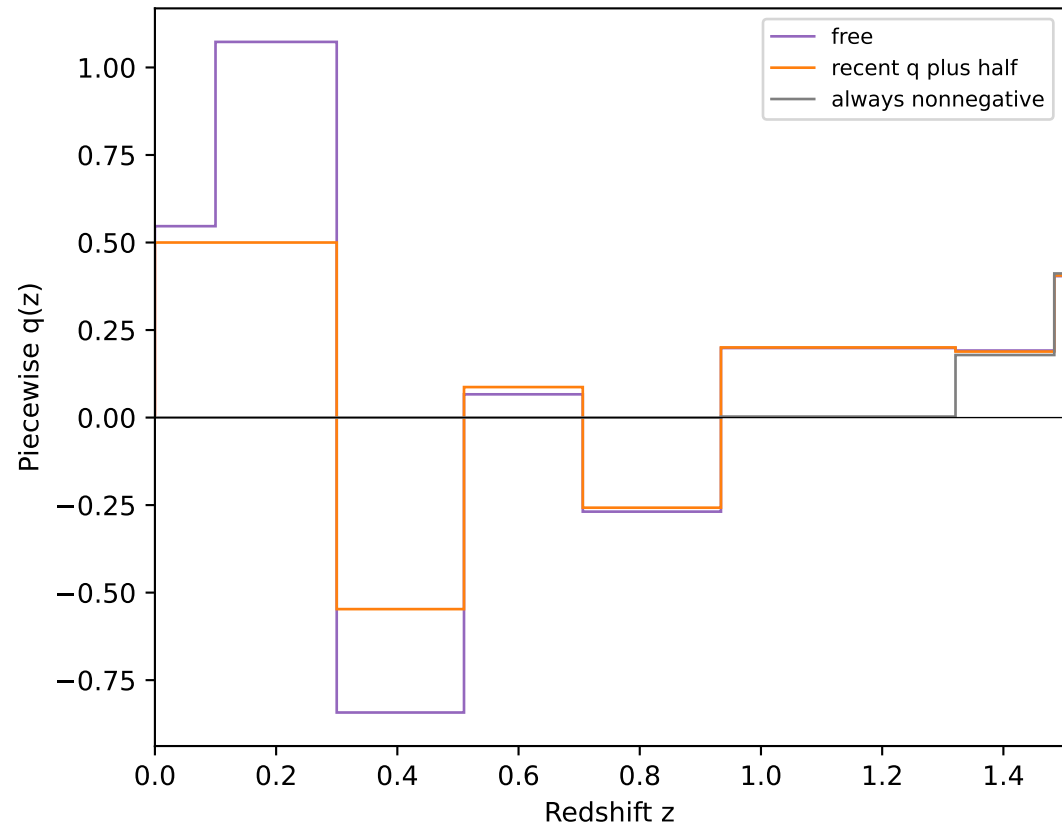
Histories fitted to BAO alone
