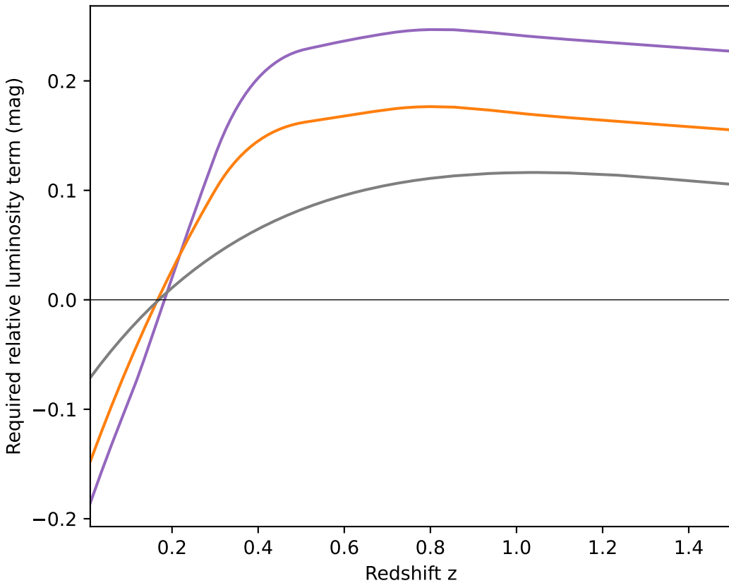
Correction to match fitted SN \Lambda CDM shape
