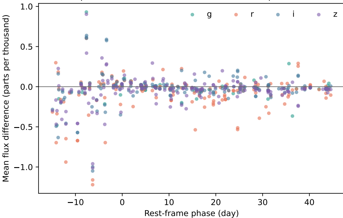
CID 1896213: local Hessian understates time uncertainty
