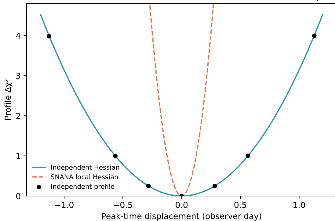
CID 1896213: local Hessian understates time uncertainty
