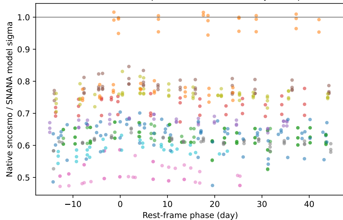
12-SN pilot: weak, heterogeneous mean-model evidence
