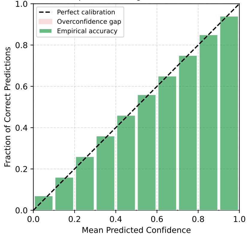
(b) After Temperature Scaling [ECE = 0.031, T^* = 1.42 ]
