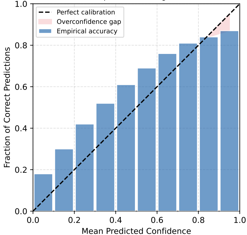
(a) Before Temperature Scaling [ECE = 0.087]
