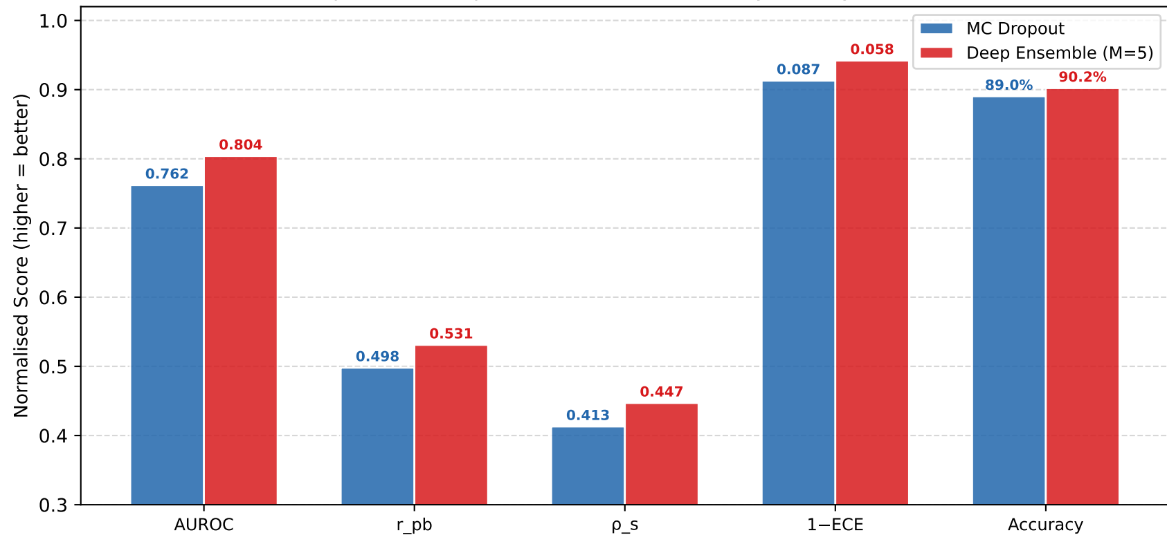
MC Dropout vs. Deep Ensemble — Uncertainty Quality (PathMNIST)
