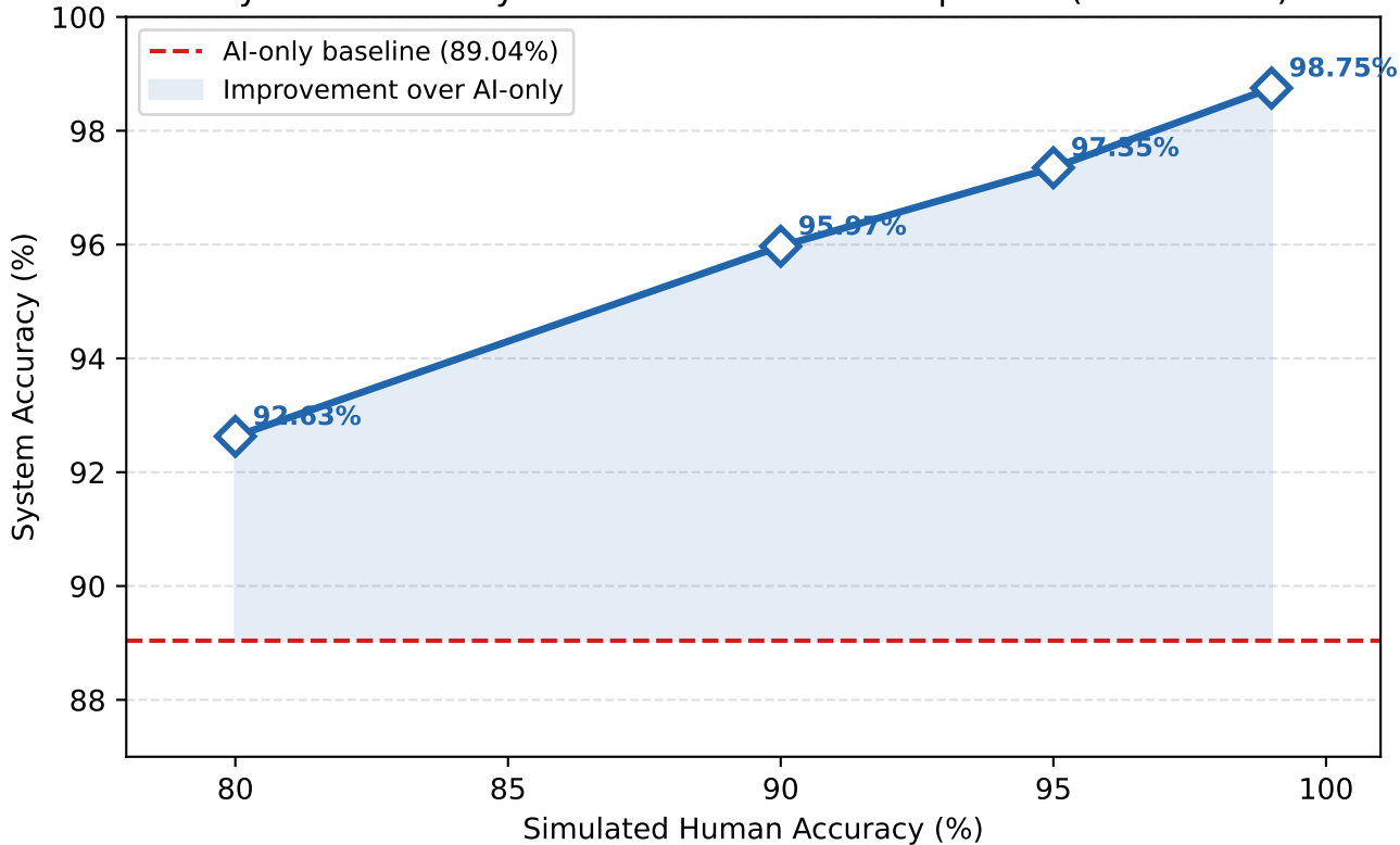
System Accuracy vs. Human Reviewer Expertise ( \tau = 0.4916 )
