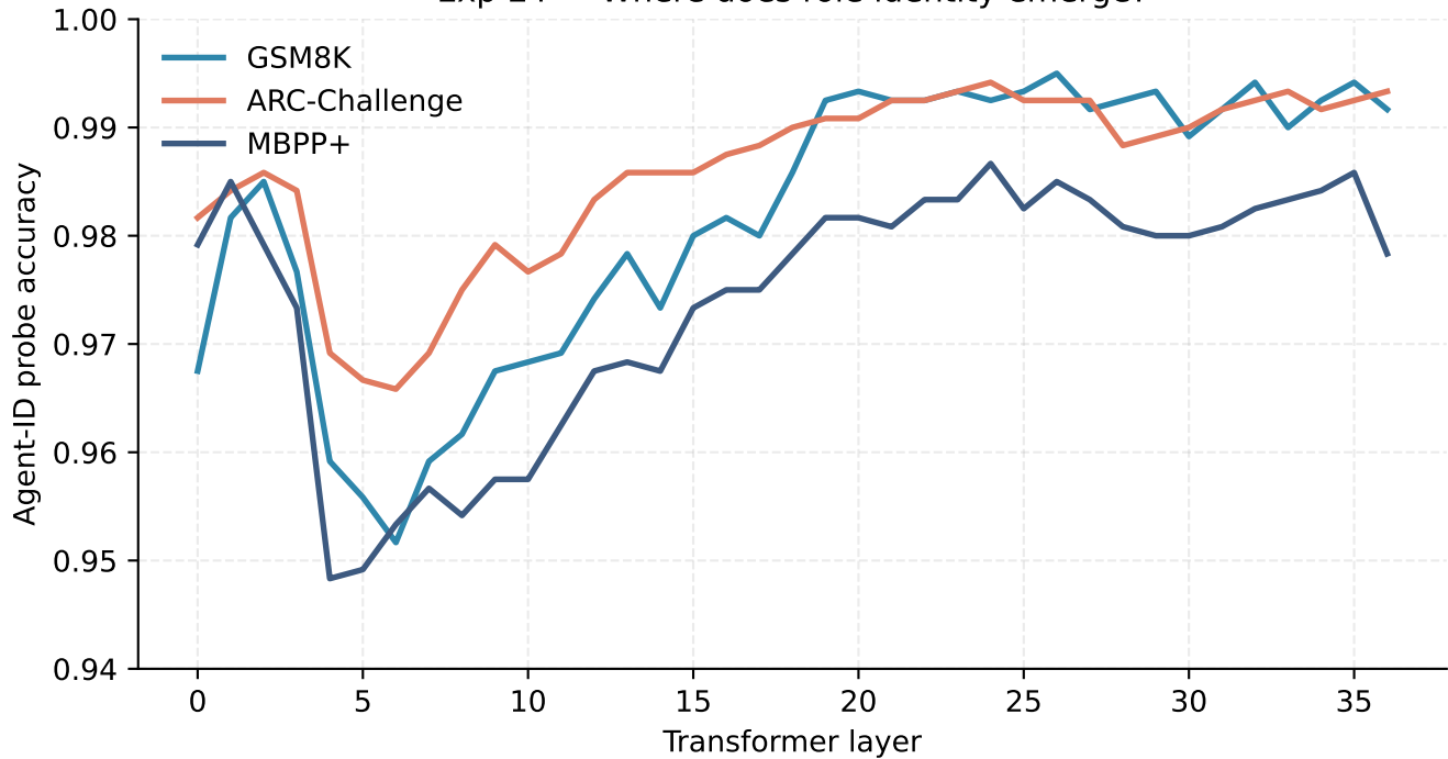
Exp E4 — Where does role identity emerge?
