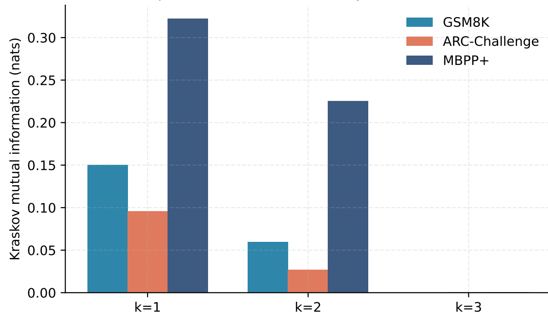
Exp F — MI(latent, label) decays across rounds
