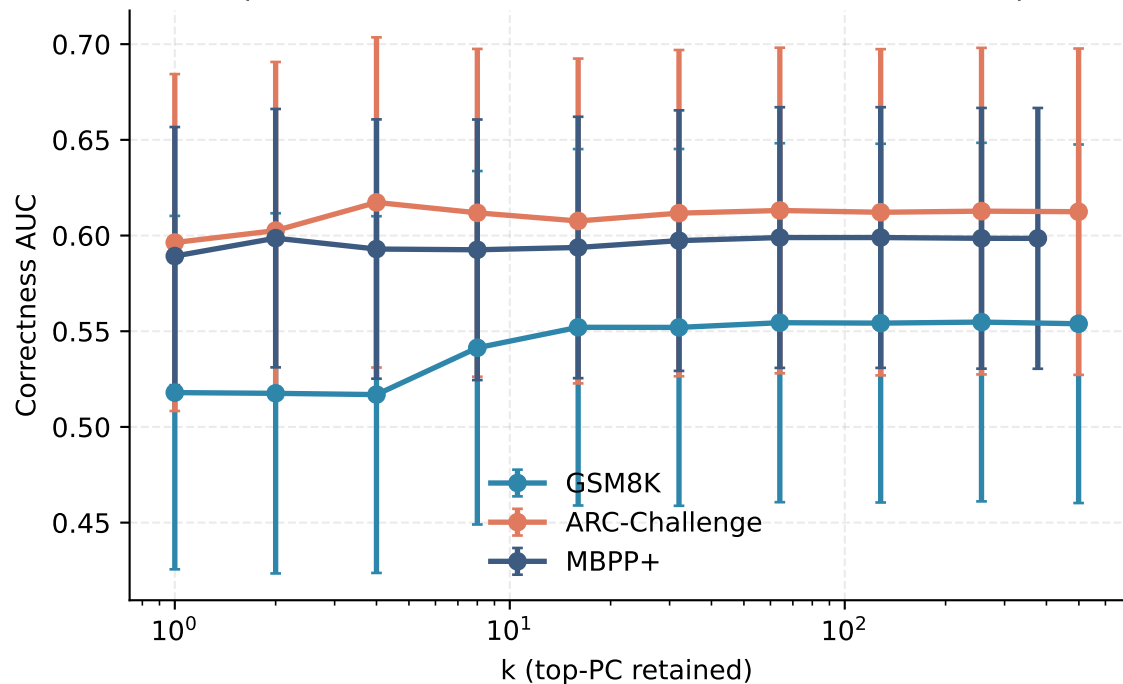
Exp F4 — Rate-distortion: AUC vs latent dimensions kept
