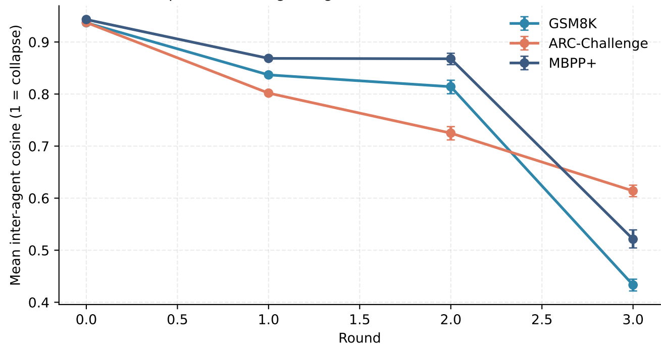
Exp G1 — Inter-agent agreement decreases over rounds
