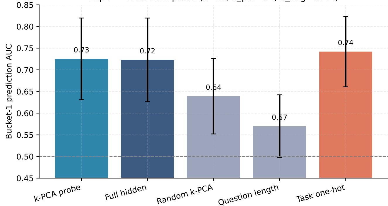
Exp P — Predictive probe (k=69, n_pos=34, n_neg=1344)
