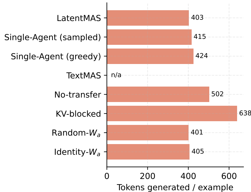
ARC-Challenge
