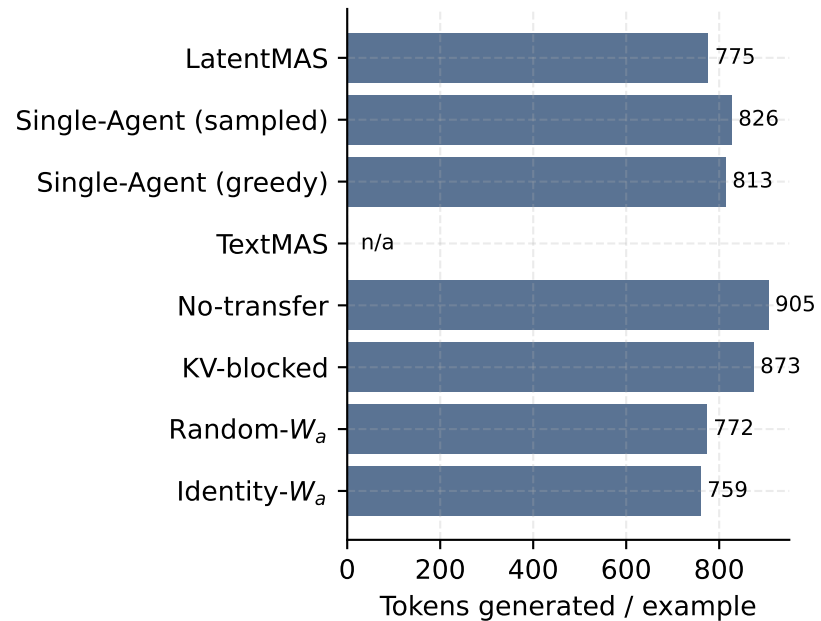
MBPP+
