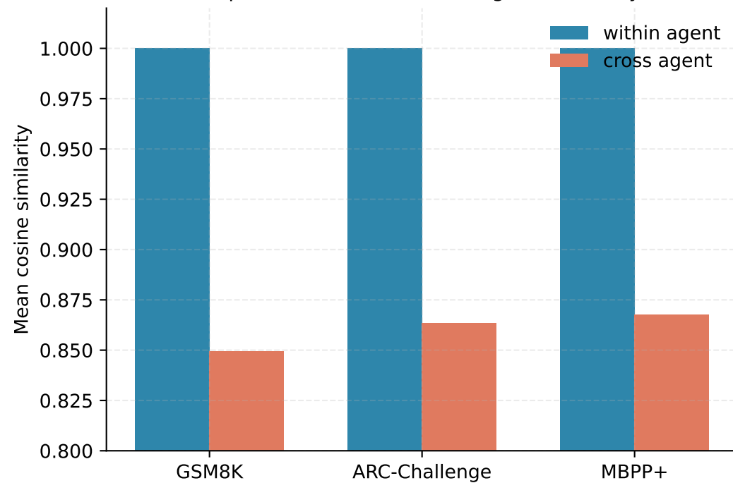
Exp E1 — Within- vs cross-agent similarity
