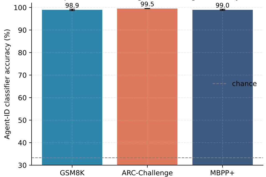
Exp E2 — Latent thoughts encode agent identity
