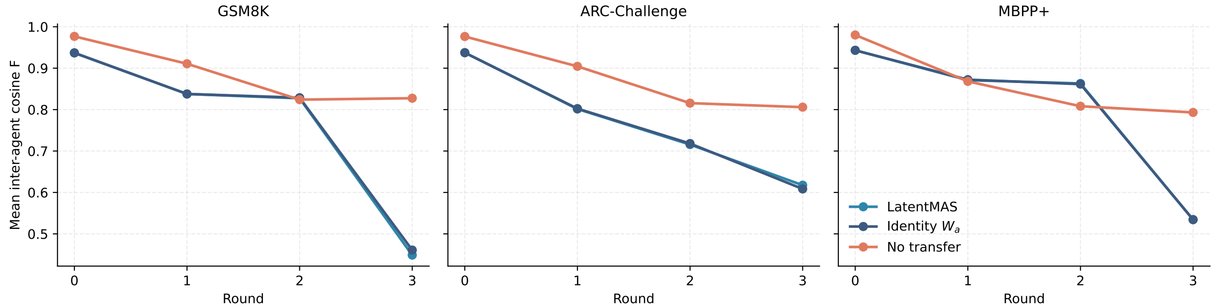
Exp M4 — 'Flocking' dynamics: convergence with vs without latent transfer
