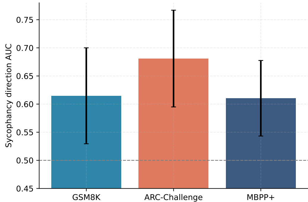
Exp N4 — Sycophancy direction predicts failure
