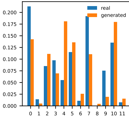
gill-color (12 cats)
