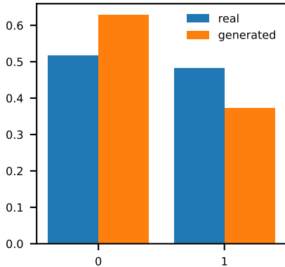
poisonous (2 cats)
