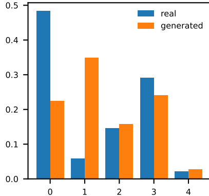
stalk-root (5 cats)
