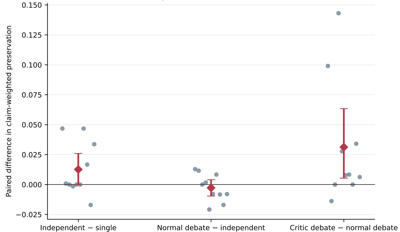
Planned paired contrasts across measures
