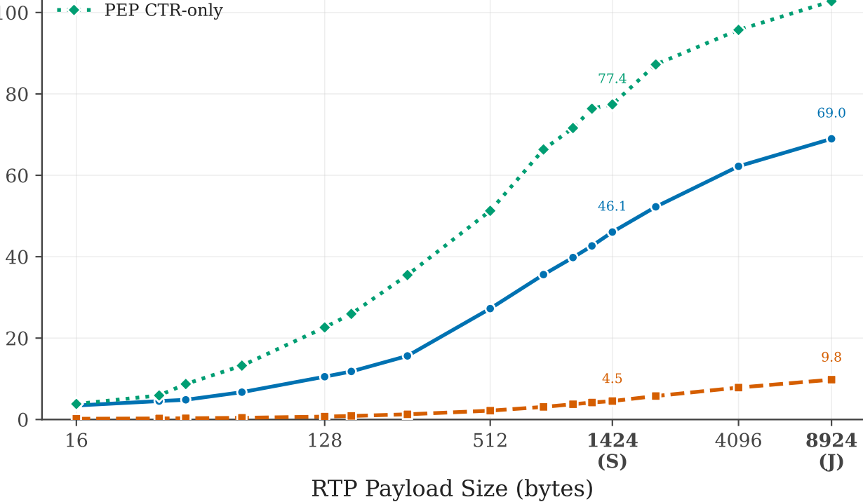
Encryption Throughput (Gbps)
