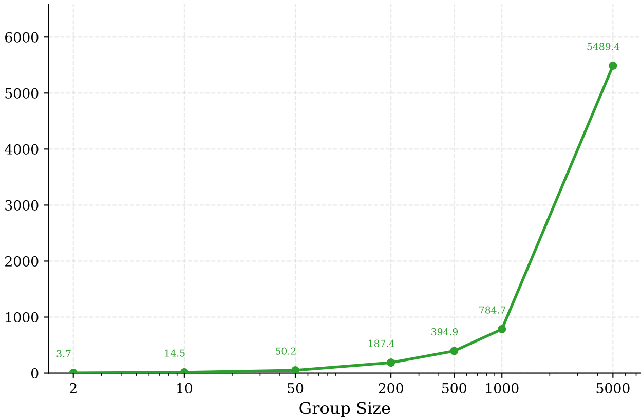
Per-Member Memory (KB)
