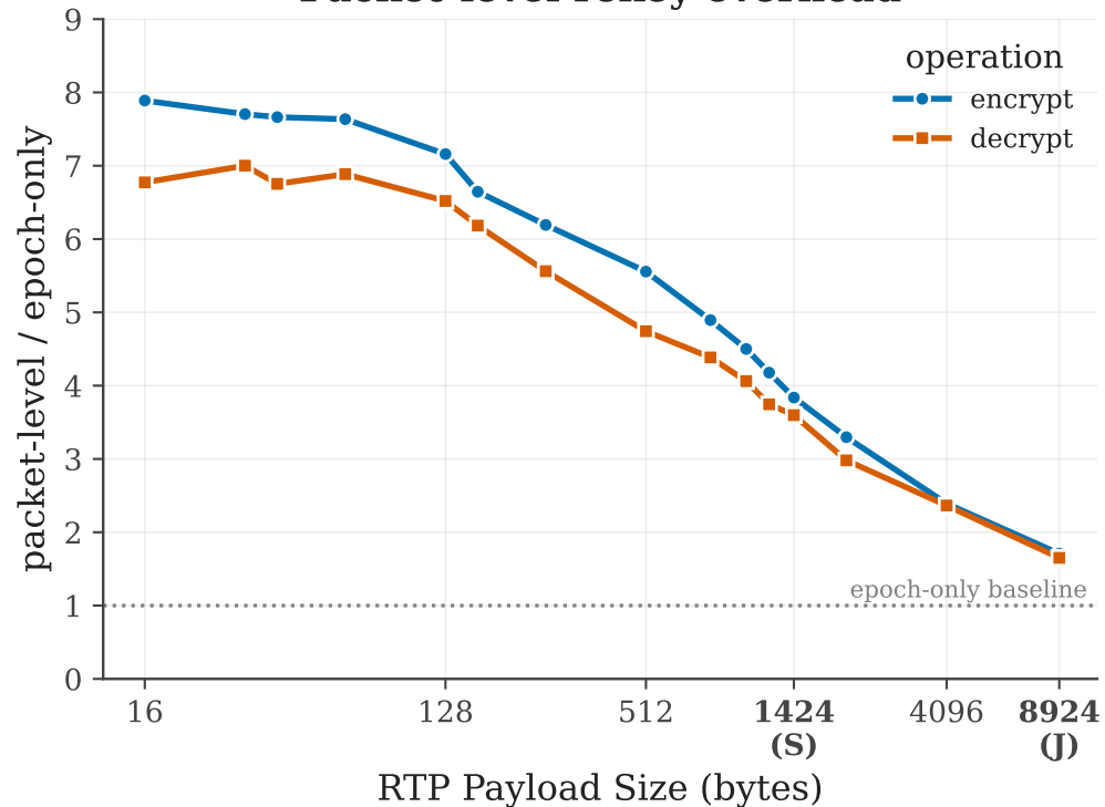
Packet-level rekey overhead
