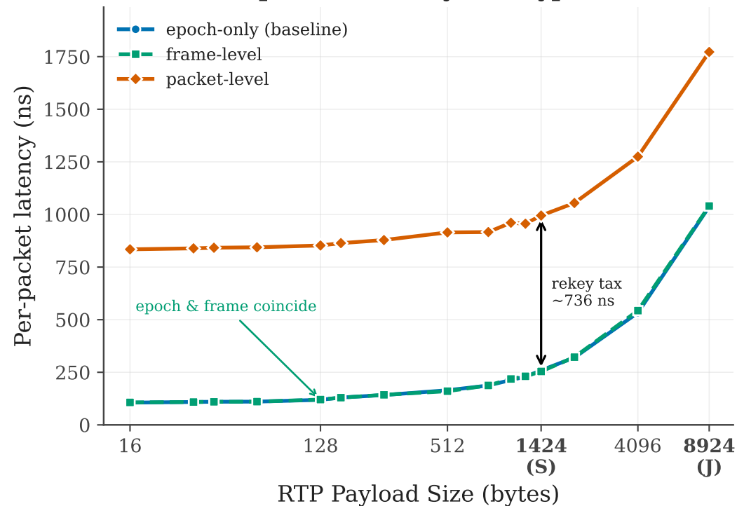
Per-packet latency (encryption)
