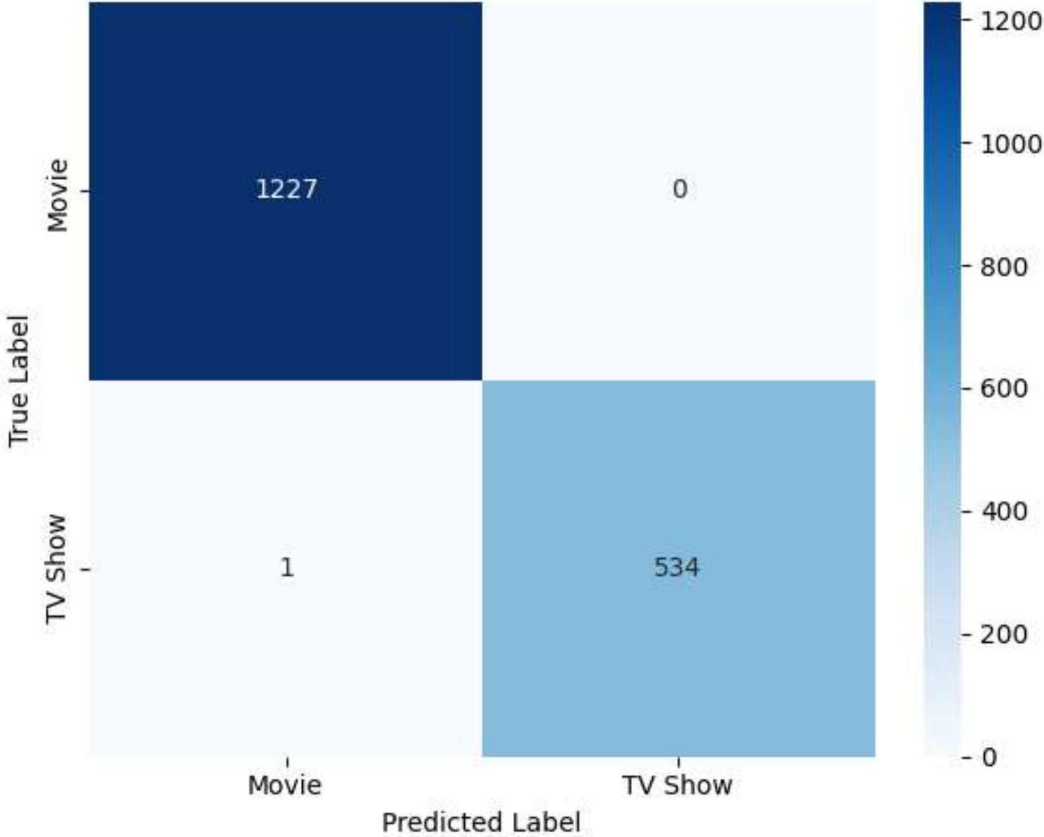
Classification Confusion Matrix
