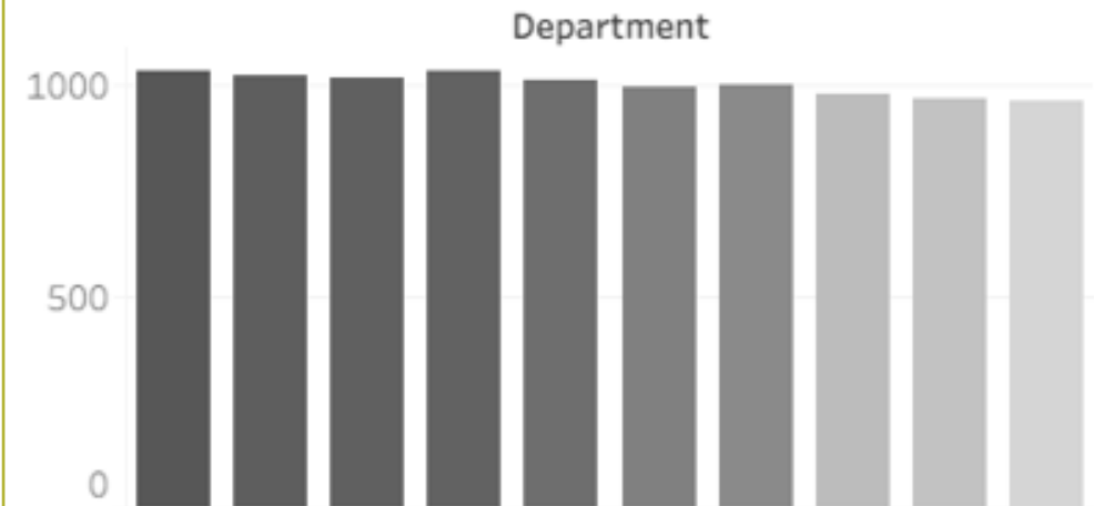
Department Comparison
