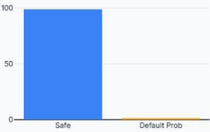
Default Probability
