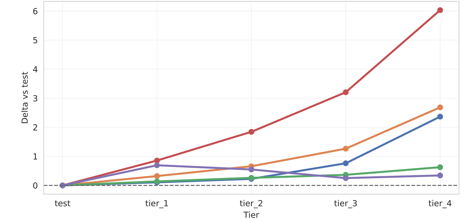
Epistemic Variance: degradation curve (delta vs test)
