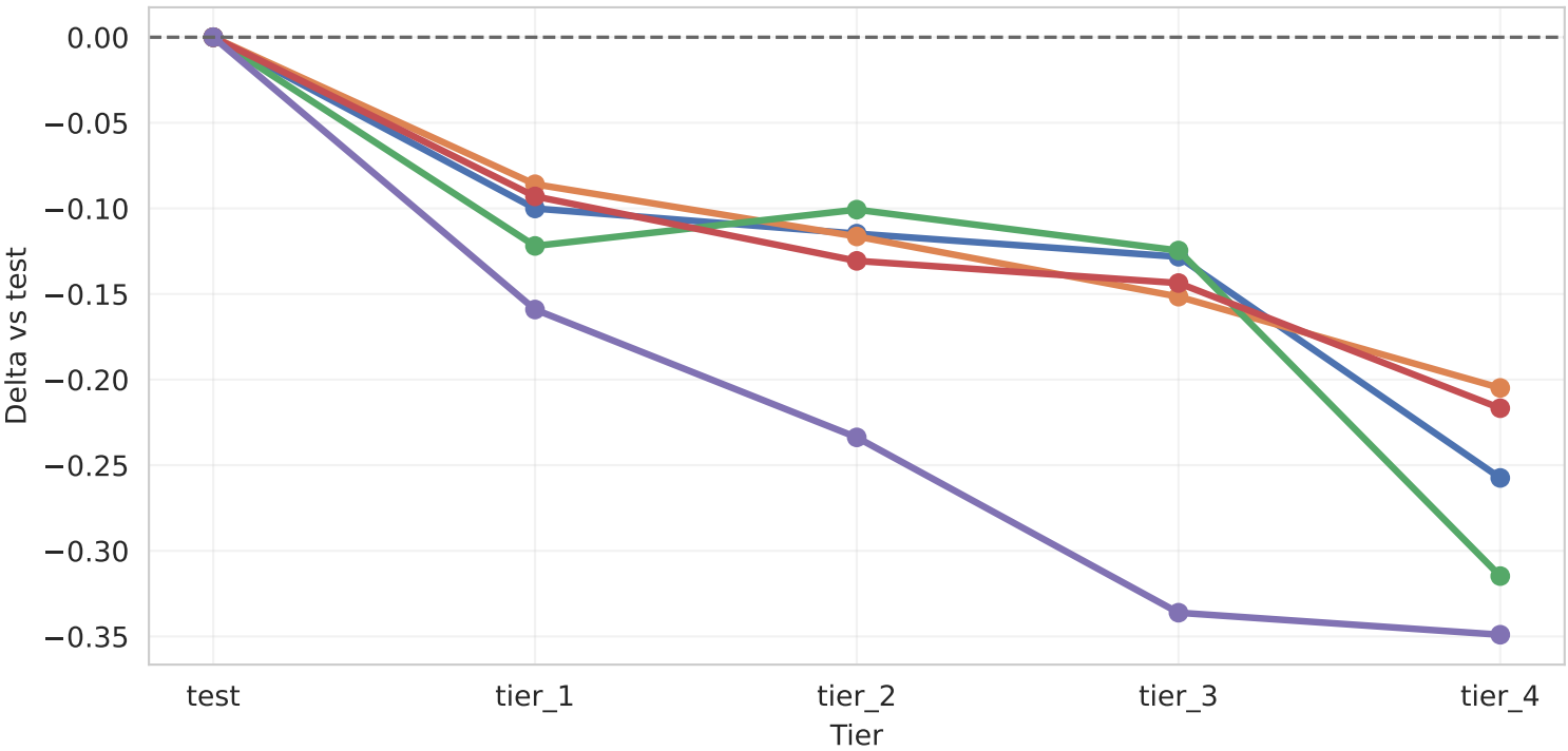
Macro-F1: degradation curve (delta vs test)
