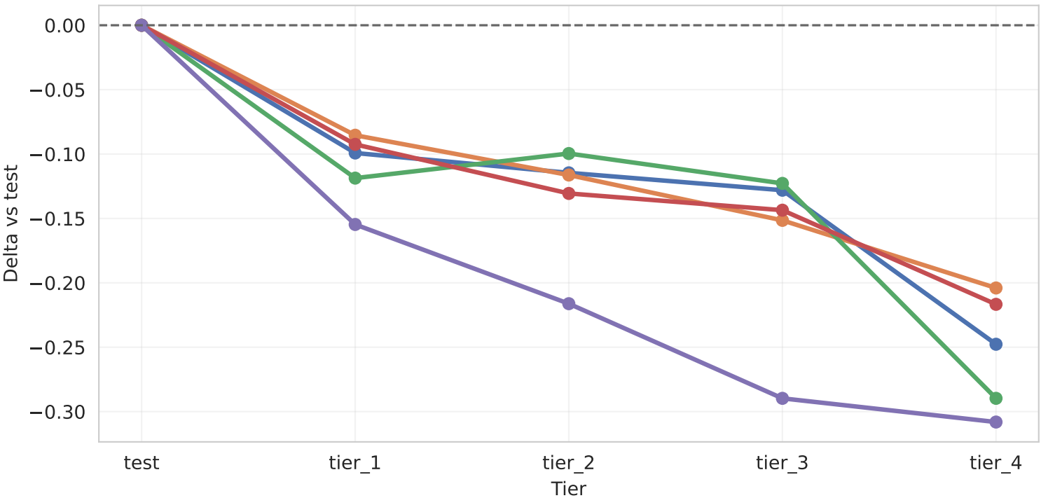
Accuracy: degradation curve (delta vs test)
