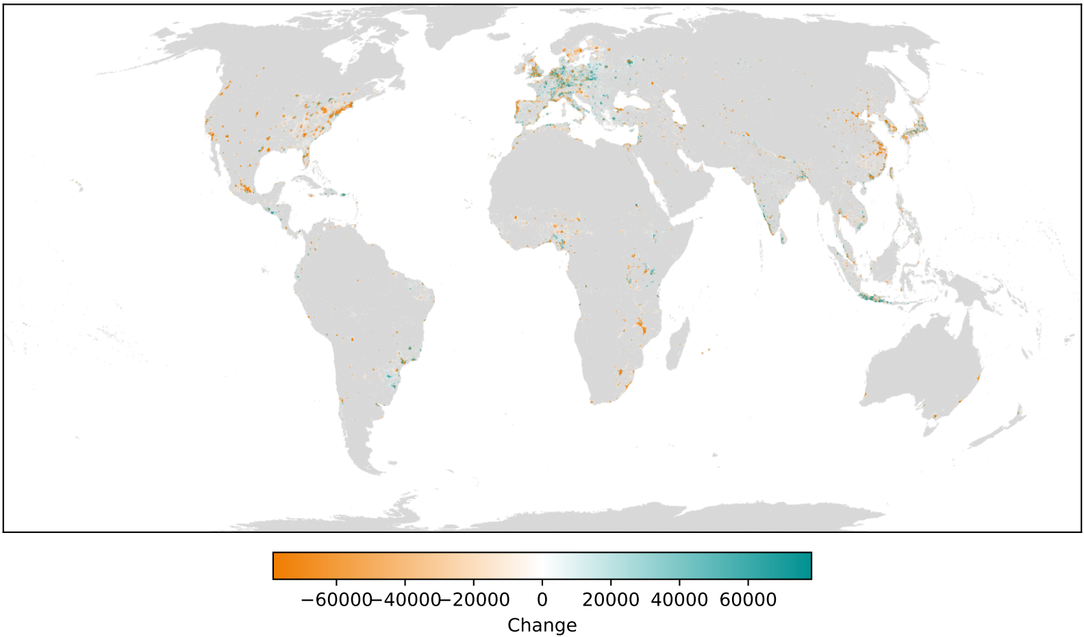
Nature Access — absolute change (1992-2020)
