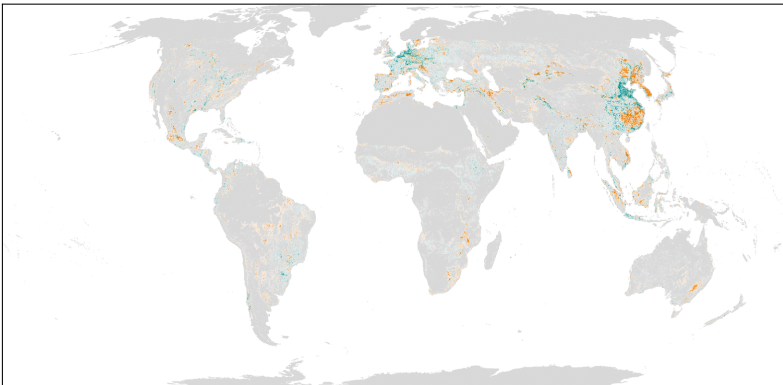
Nitrogen Export — absolute change (1992-2020)
