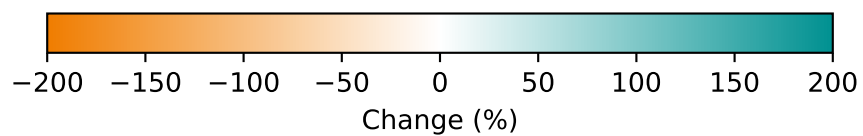
Nature Access — relative hotspots (top 5% most severe decline)
