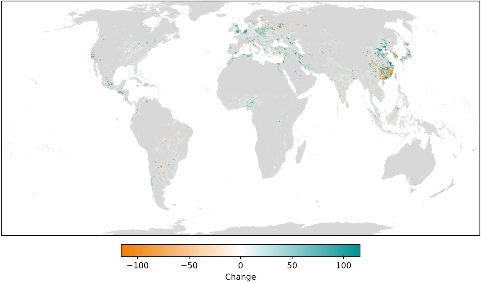
Pollination — absolute change (1992-2020)
