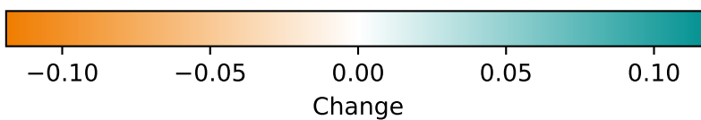
Nitrogen Retention Ratio — absolute hotspots (top 5% most severe decline)
