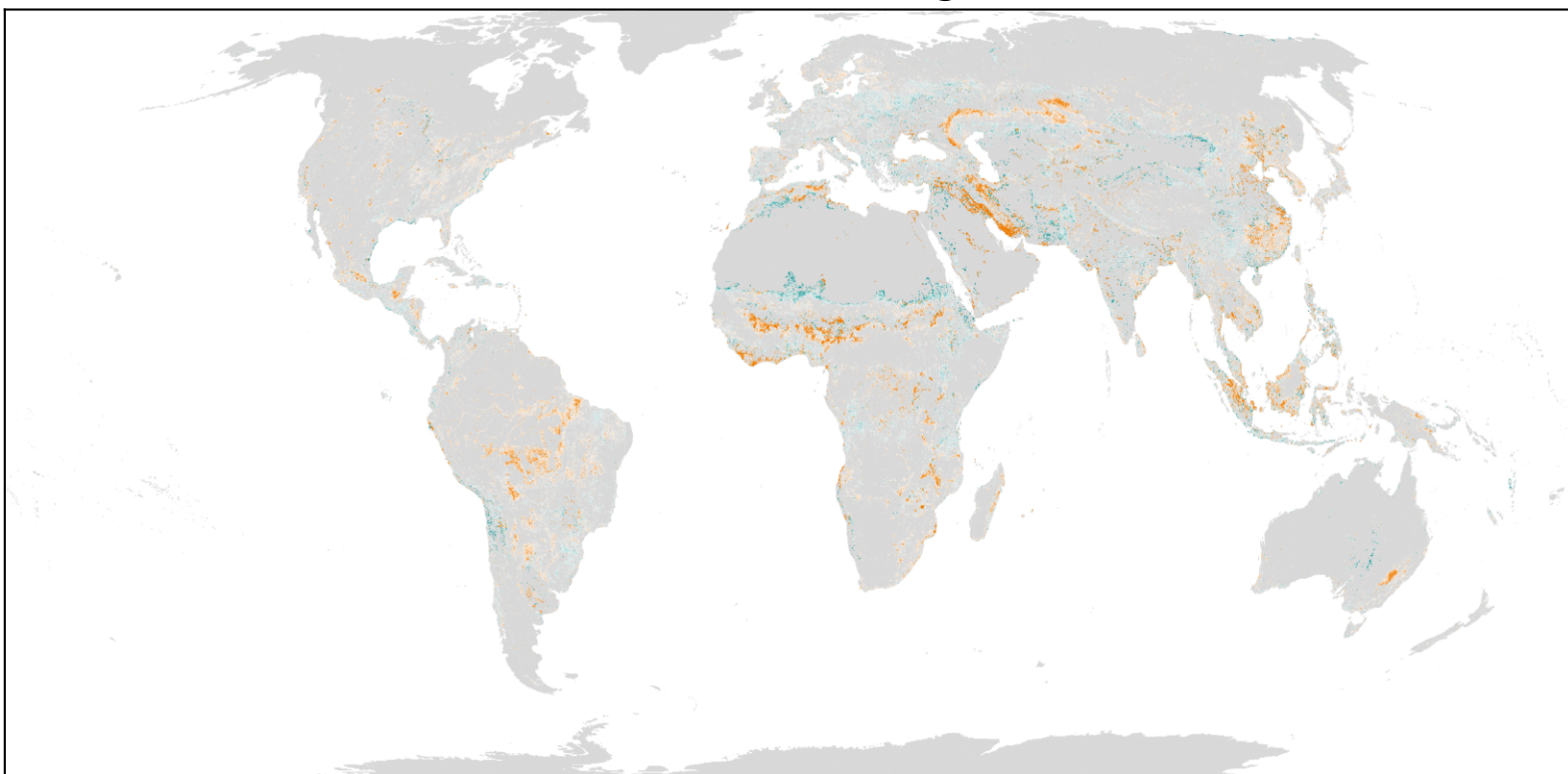
Nature Access — relative change (1992-2020)
