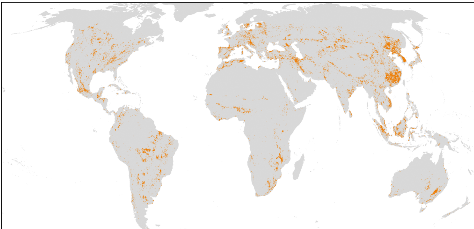
Nitrogen Export — absolute hotspots (top 5% most severe decline)
