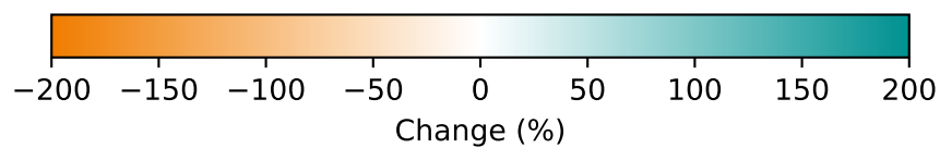
Coastal Risk Reduction Ratio — relative hotspots (top 5% most severe decline)
