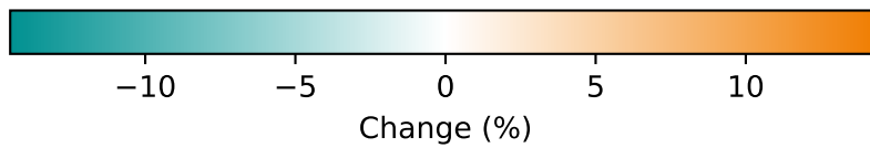
Coastal Risk — relative hotspots (top 5% most severe decline)
