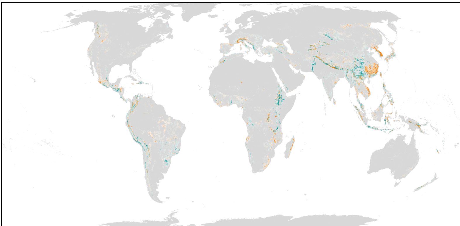
Sediment Export — absolute change (1992-2020)
