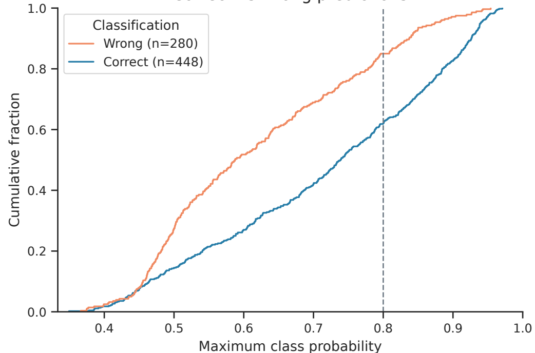
Correct vs wrong predictions
