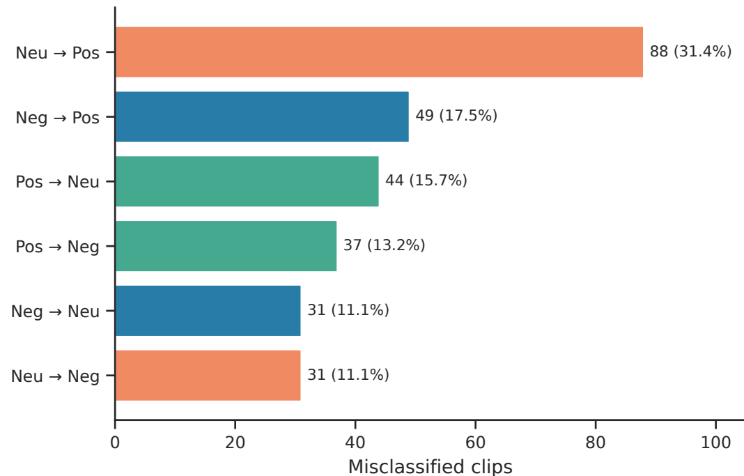
All 280 errors / validation
