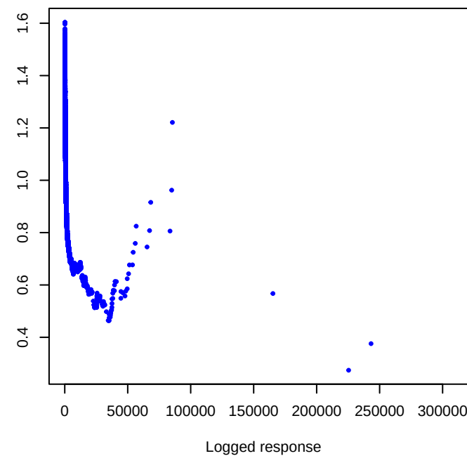
Pareto derivative plot
