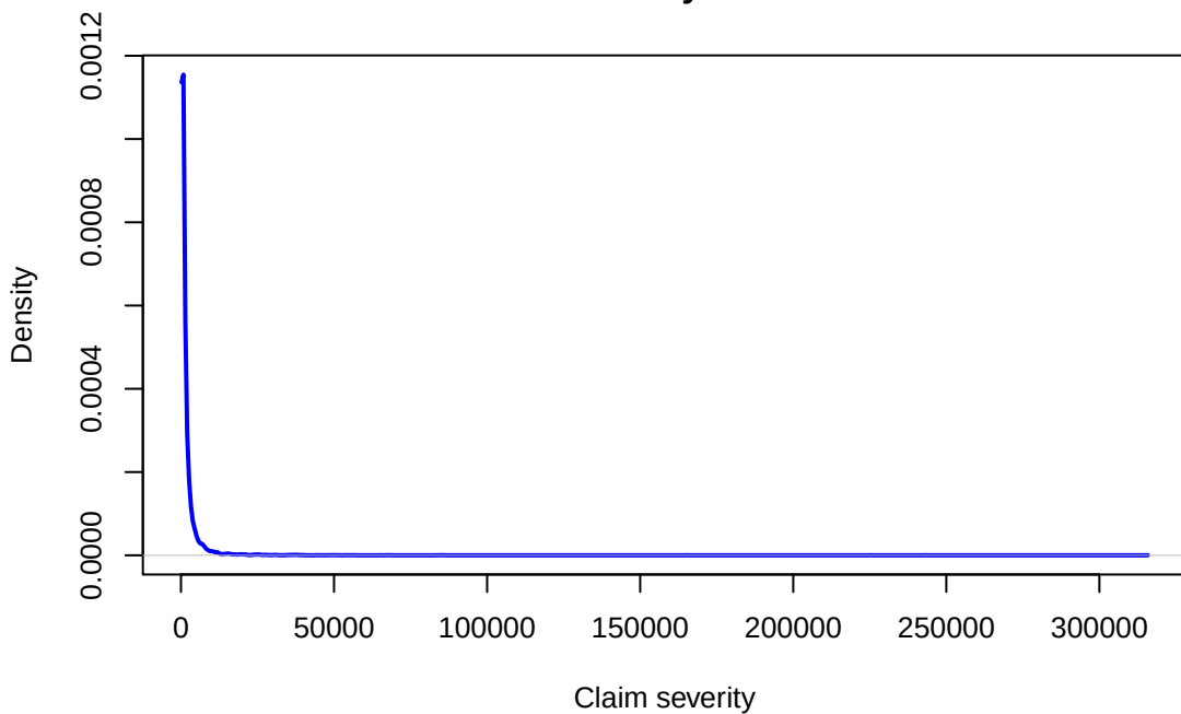
Kernel density estimator
