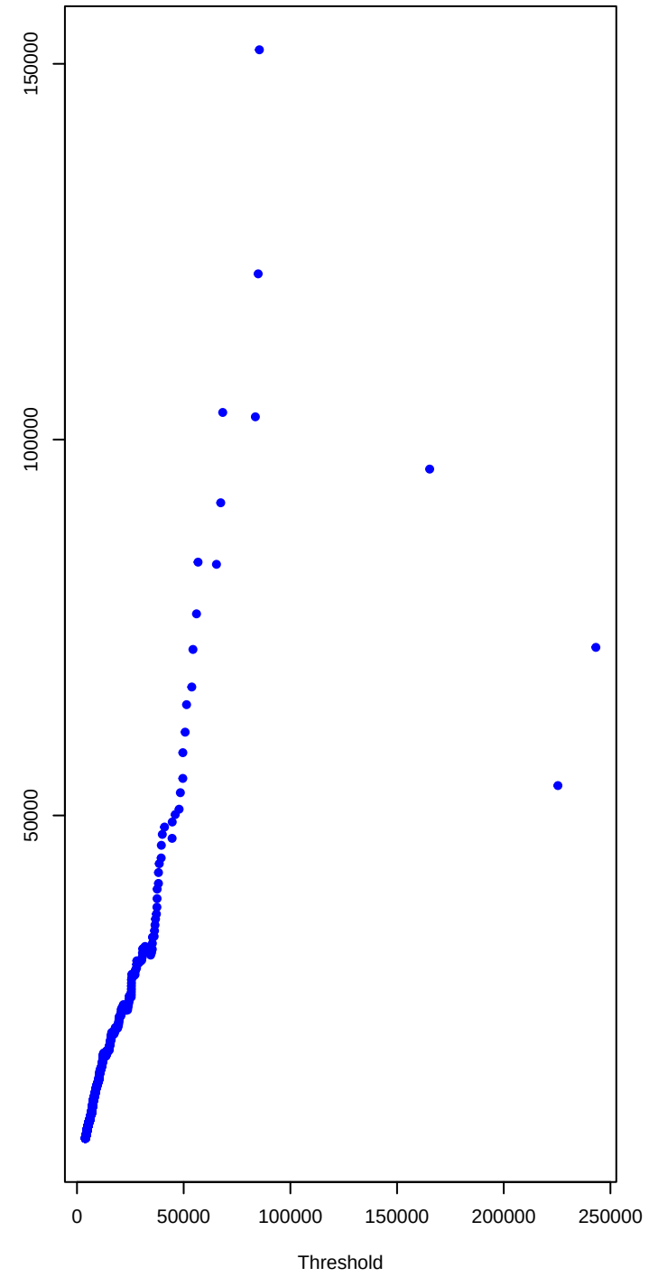
Mean excess plot
