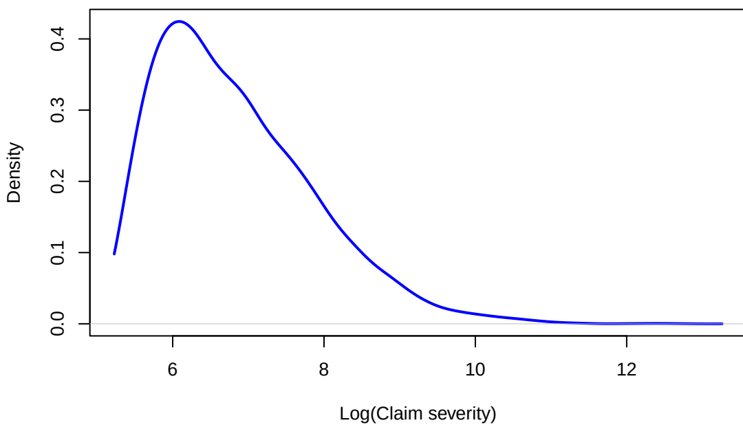
Kernel density estimator (Logarithm)
