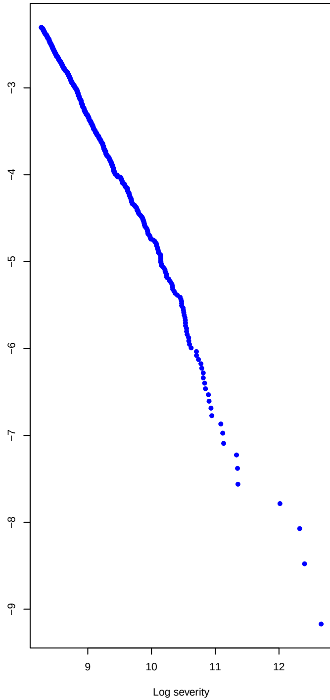
Log tail of distribution
