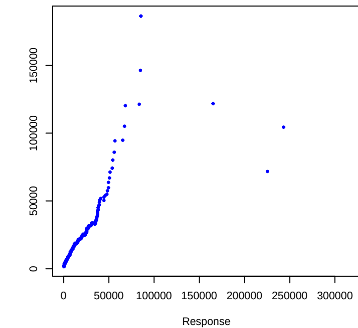
Exponential derivative plot
