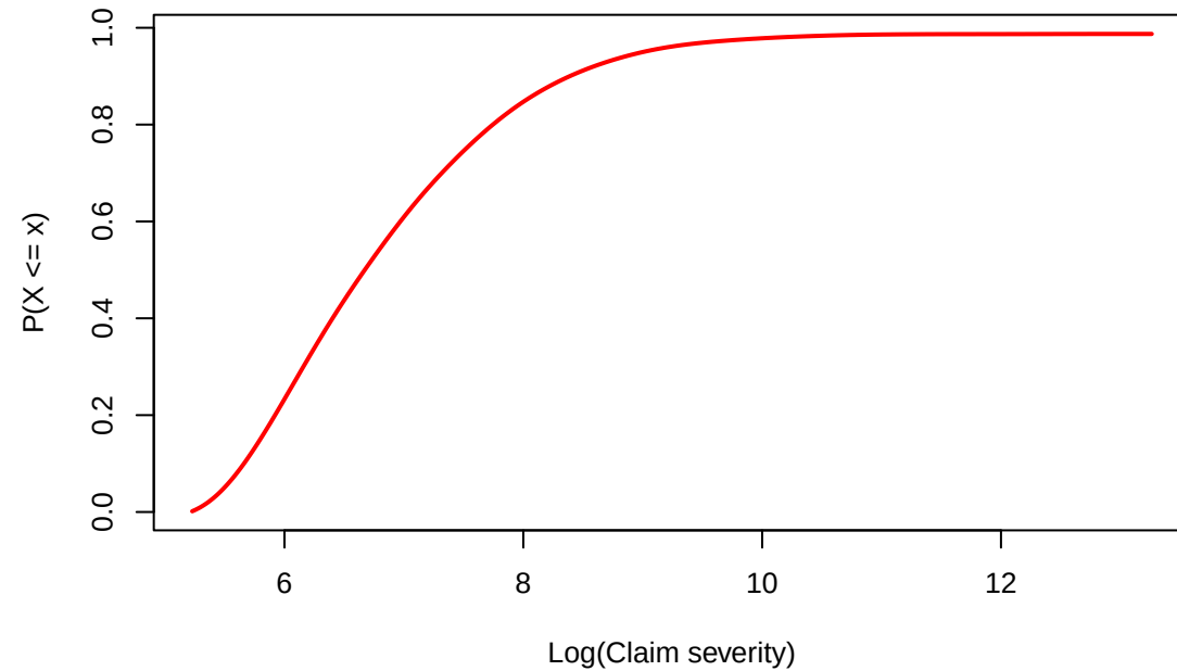
Kernel CDF (Logarithm)
