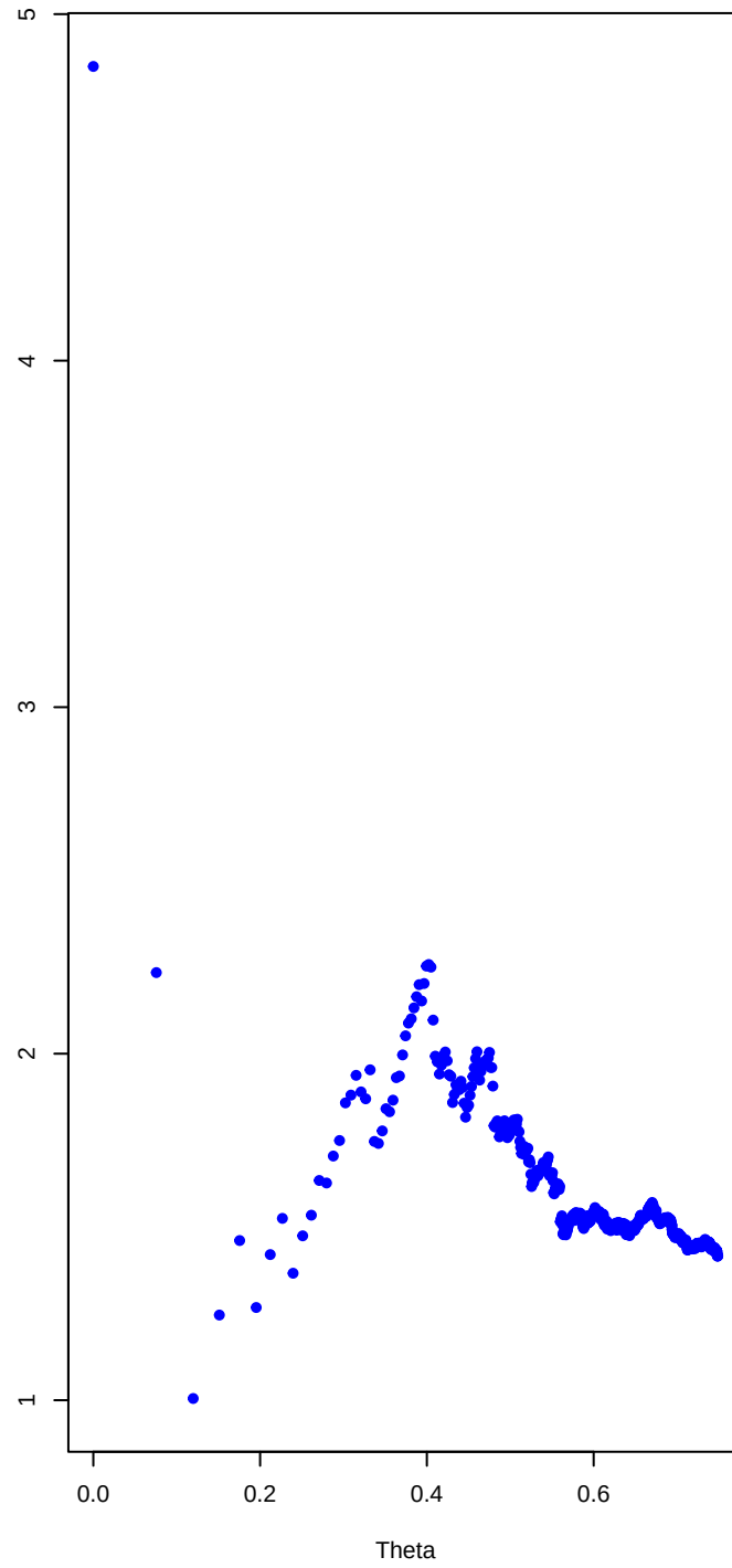
Hill estimator of tail index alpha
