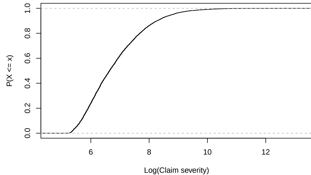
Empirical CDF (Logarithm)
