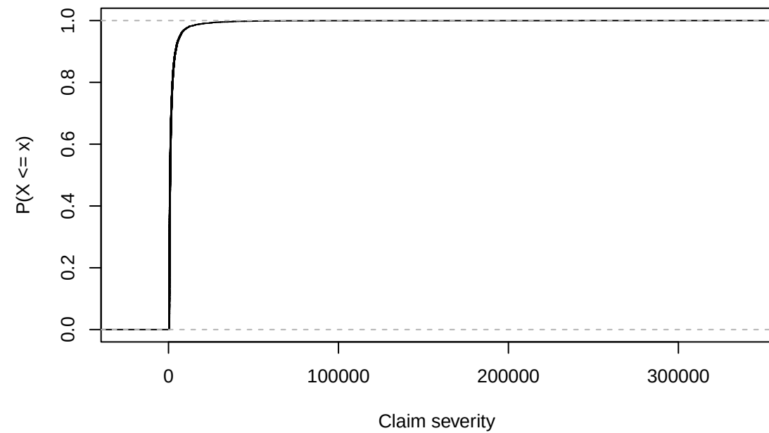
Empirical CDF (Original)
