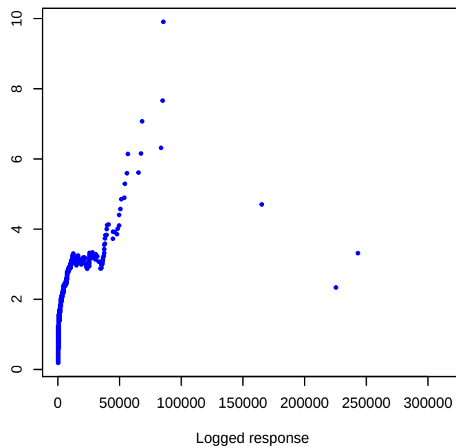
Weibull derivative plot
