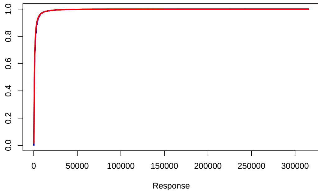
Distribution function
