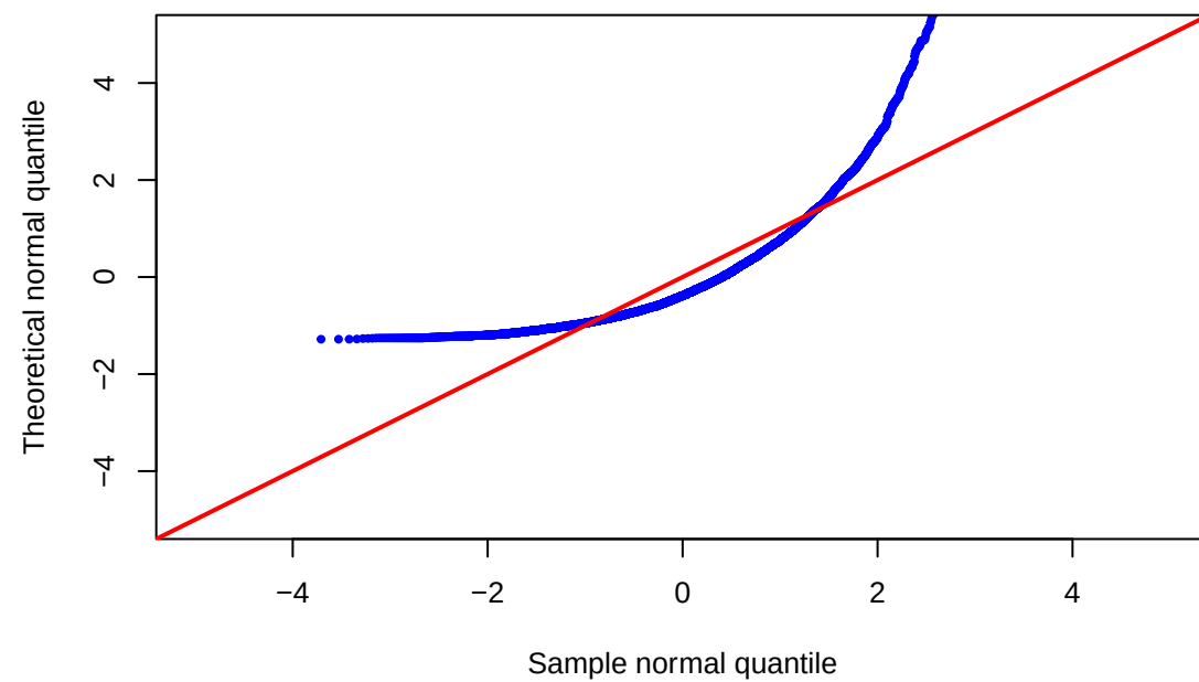
QQ plot
