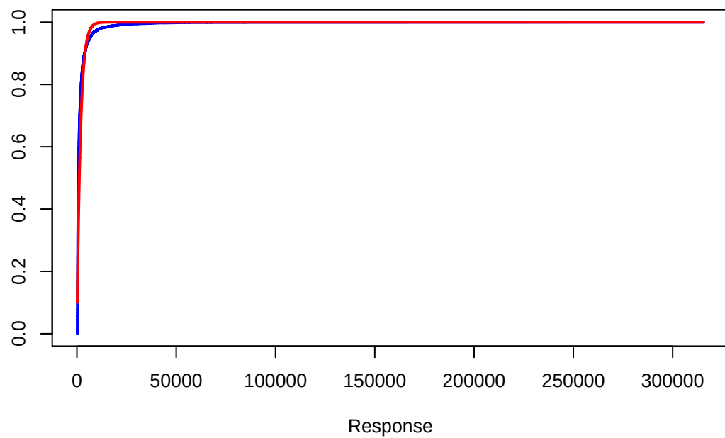
Distribution function
