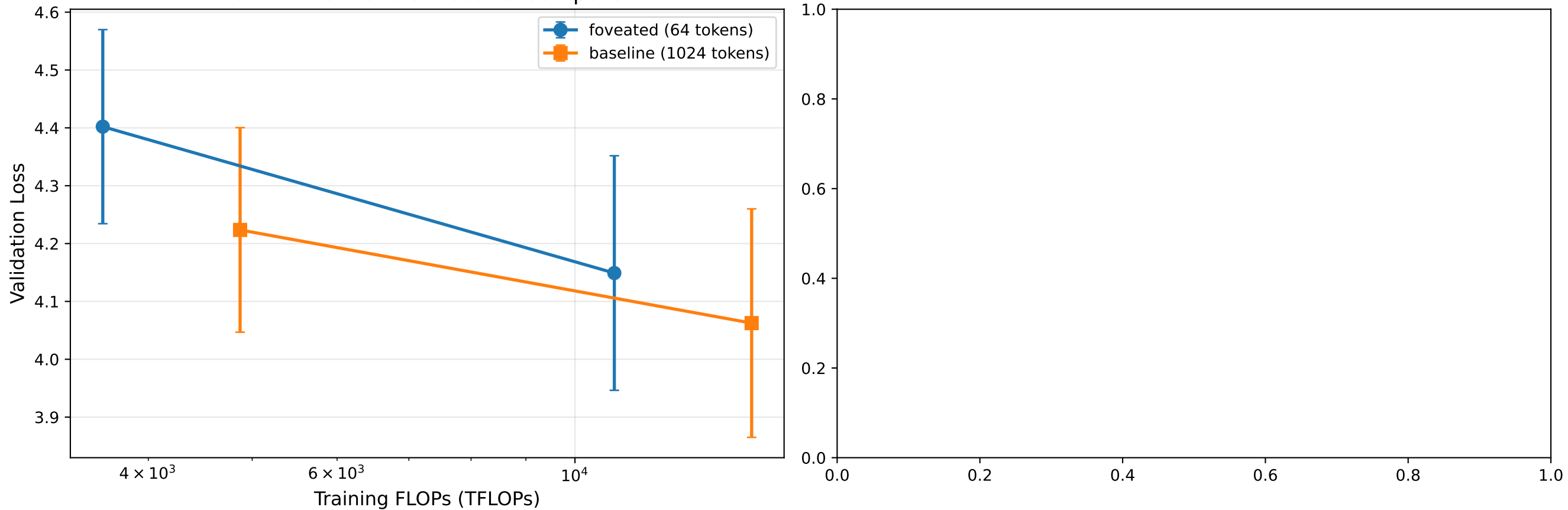
64-Frame Models: Loss vs Compute
