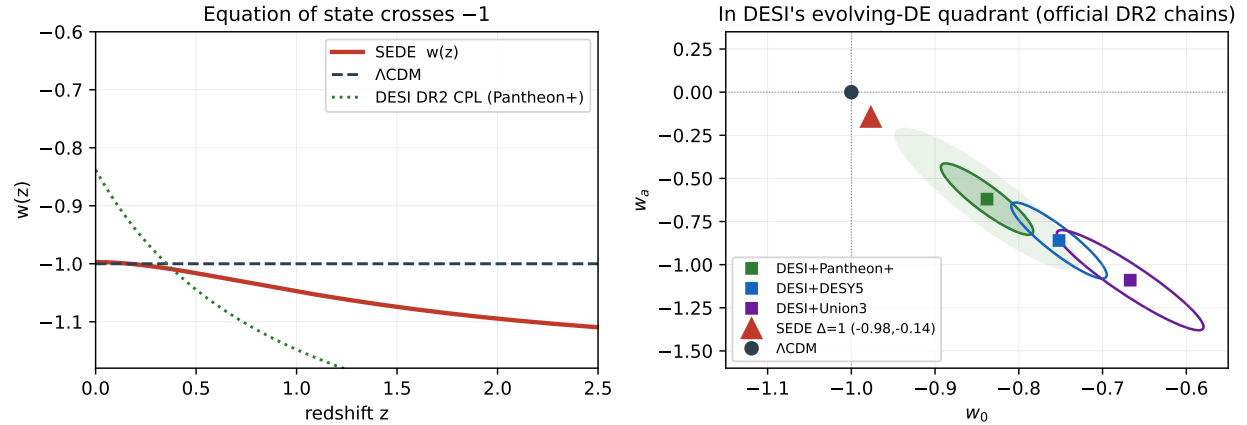
Figure 4. The equation of state. Left: the canonical SEDE-H fluid w(z) (red) crosses -1 near z \approx 0 and dips into the phantom regime ( \approx -1.08 by z \approx 2 ), the same sense as DESI DR2's CPL fit (green) and distinct from \Lambda CDM (dashed). Right: the (w_0, w_a) plane — SEDE sits between \Lambda CDM and the DESI DR2 w_0 w a CDM contour, in the evolving-dark-energy quadrant. The crossing is not imposed; it is where the expansion and horizon-entropy-production terms in 1 + w balance (Result 13).
