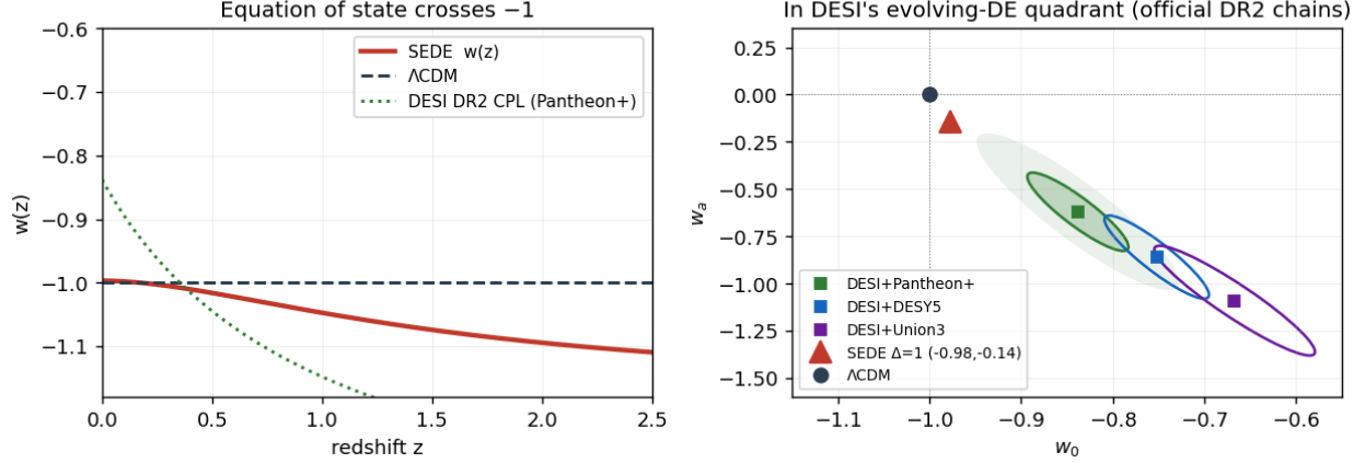
Figure 4. The equation of state. Left : the canonical SEDE-H fluid w(z) (red) crosses -1 near z \approx 0 and dips into the phantom regime ( \approx -1.08 by z \approx 2 ), the same sense as DESI DR2's CPL fit (green) and distinct from \Lambda CDM (dashed). Right : the (w_0, w_a) plane — SEDE sits between \Lambda CDM and the DESI DR2 w_0 w a CDM contour, in the evolving-dark-energy quadrant. The crossing is not imposed; it is where the expansion and horizon-entropy-production terms in 1 + w balance (Result 13).
