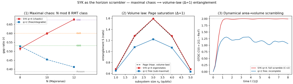
Figure G1. SYK as the horizon scrambler ( q=4 chaotic vs q=2 integrable control). Left : gap ratio climbs through the N-mod-8 RMT classes (GOE \rightarrow GUE \rightarrow GSE) — the certificate of maximal chaos. Centre : eigenstate entanglement saturates the Page value. Right : the OTOC scrambles completely ( C \rightarrow 2 ). This fixes the state , not the counting.
