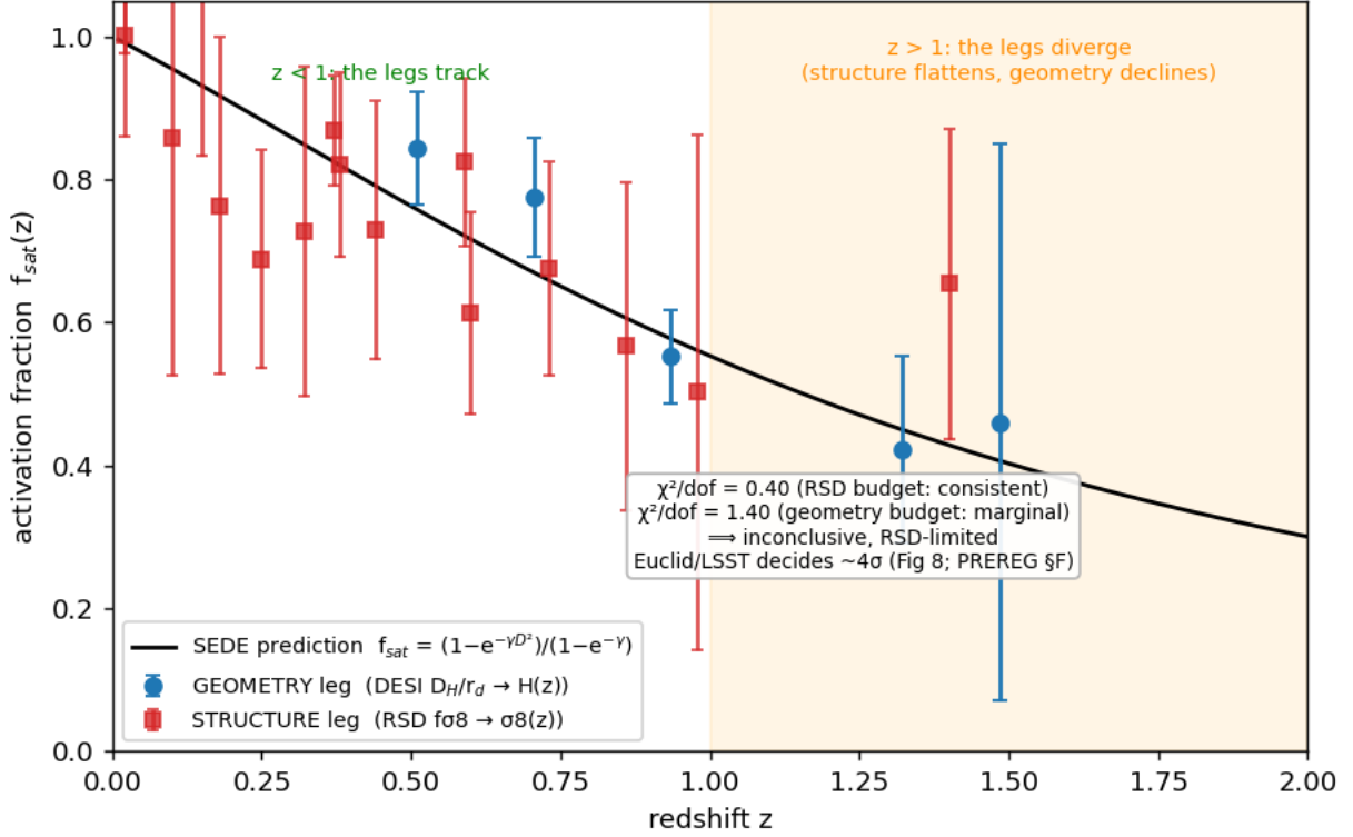
E1 — the structure-sourcing mechanism on CURRENT data SEDE's founding claim: the two legs should coincide
