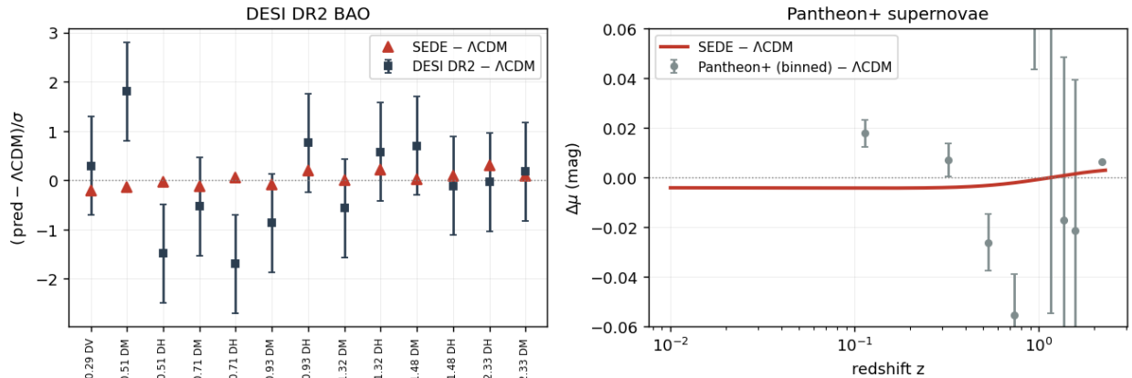
The model fits the data: DESI BAO and Pantheon+ residuals vs \Lambda CDM
