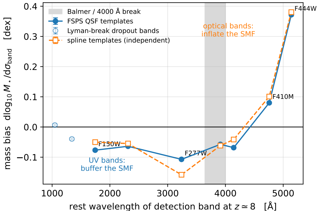
Sign of the mass-selection bias vs selection band
