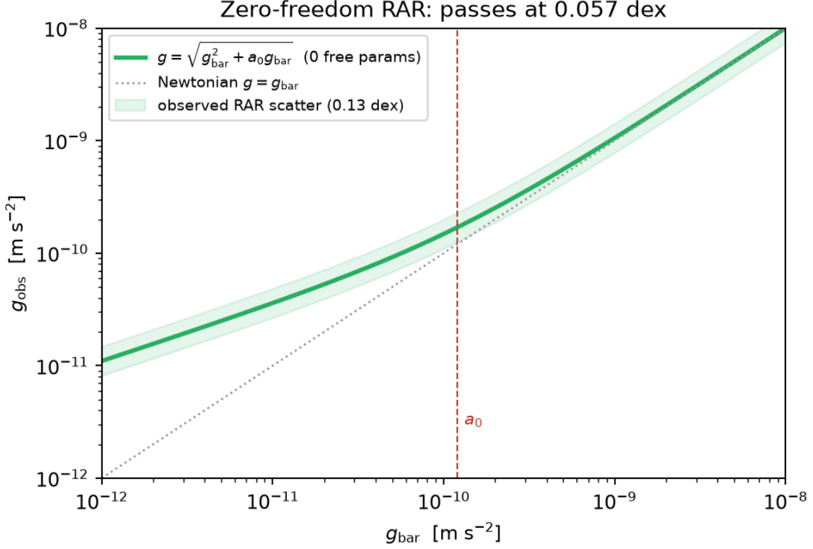
FIG. 2. The zero-freedom radial acceleration relation. The KMS-tilt interpolation g_{\text{obs}} = \sqrt{g_{\text{bar}}^2 + a_0 g_{\text{bar}}} (green) has no shape parameter; it passes the observed RAR at 0.057 dex, inside the 0.13-dex scatter (band). a_0 is the only scale, and in the rate branch it is set by H(z) .
