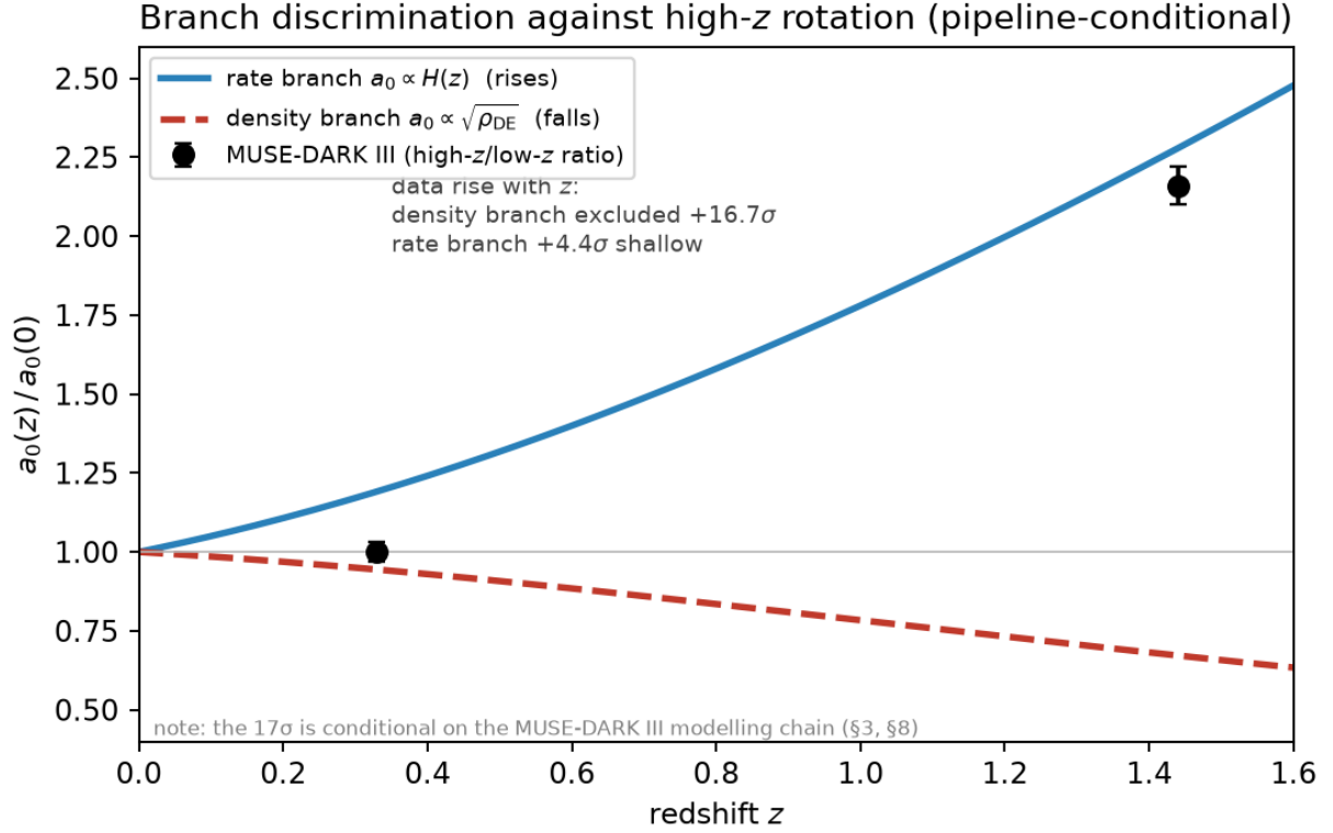
FIG. 1. Branch discrimination against high- z rotation. The rate branch a_0 \propto H(z) rises with redshift (blue), tracking the MUSE-DARK III trend (ratio 2.16 \pm 0.06 over z = 0.33 \rightarrow 1.44 ); the density branch a_0 \propto \sqrt{\rho_{\text{DE}}} falls (red), the wrong sign — excluded at +16.7\sigma . The rate branch is +4.4\sigma shallow. The significance is conditional on the MUSE-DARK III modelling chain (§III, §VIII).
