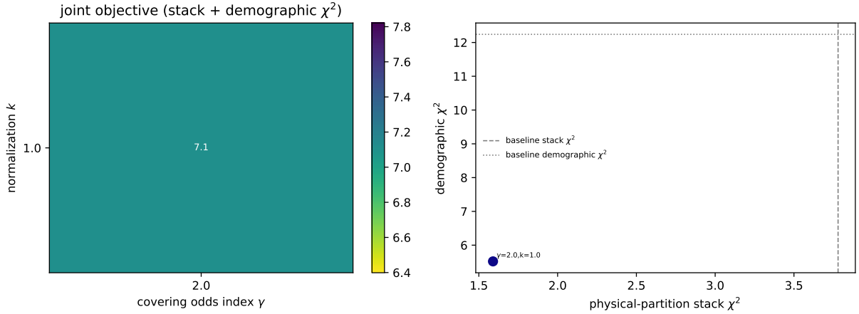
Figure 2. Joint scan of the covering law under the fiducial metric. Left: joint objective (flux-stacked line-ratio \chi^2 plus z \leq 7.5 demographic \chi^2 ; logarithmic color scale) over the evaluated (\gamma, k) cells; the preferred point is the unit-normalization quadratic. Right: spectral versus demographic components for all evaluated points. The objective is a descriptive sum; no probabilistic reading of \Delta values is intended.
