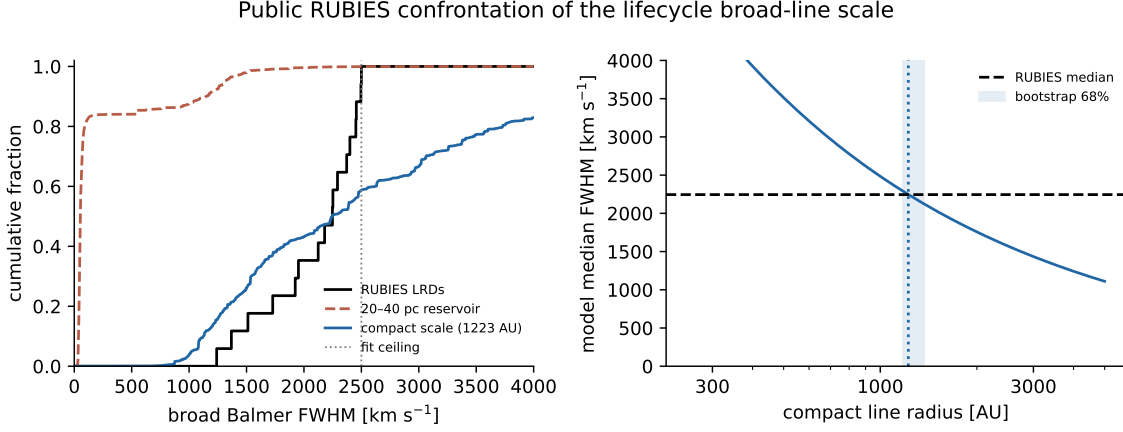
Figure 3. RUBIES broad Balmer width confrontation under the fitted covering law. Left: cumulative width distributions; the dotted vertical line marks the 2500 km s -1 ceiling imposed in the published broad-component fits (the model CDFs are not truncated). The dashed curve shows the superseded 20–40 pc reservoir-scale width model for reference. Right: descriptive compact-scale calibration; the model median matches the observed median at 5.9 \times 10^3 AU with a substantial electron-scattering contribution.
