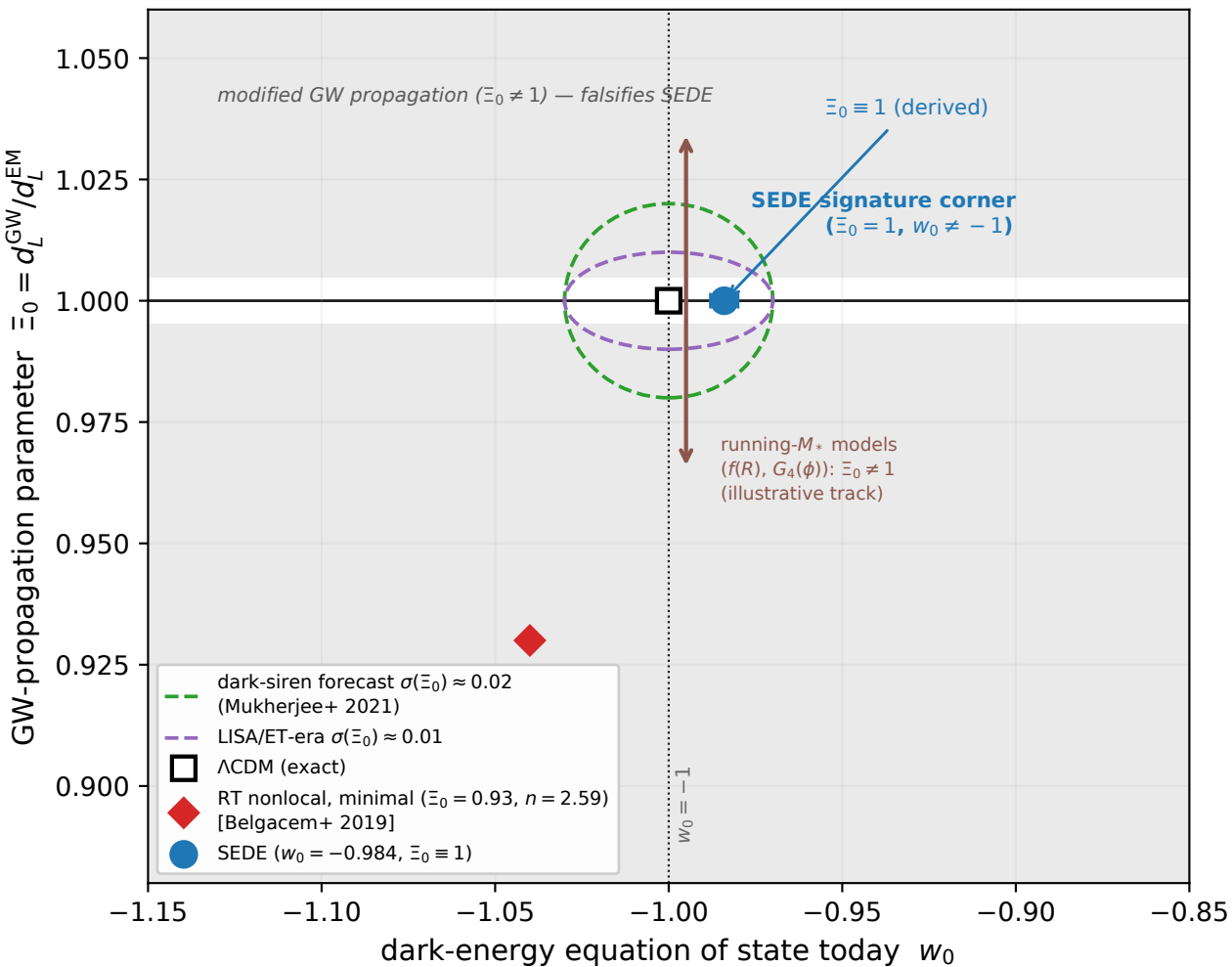
The (\Xi_0, w_0) discriminant plane
