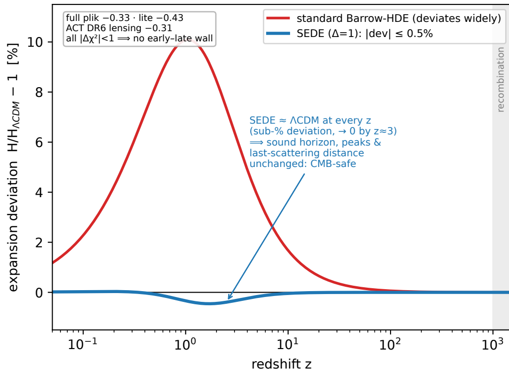
SEDE deforms only the late expansion \rightarrow 0 by z \approx 3 (BBN/recombination standard)
