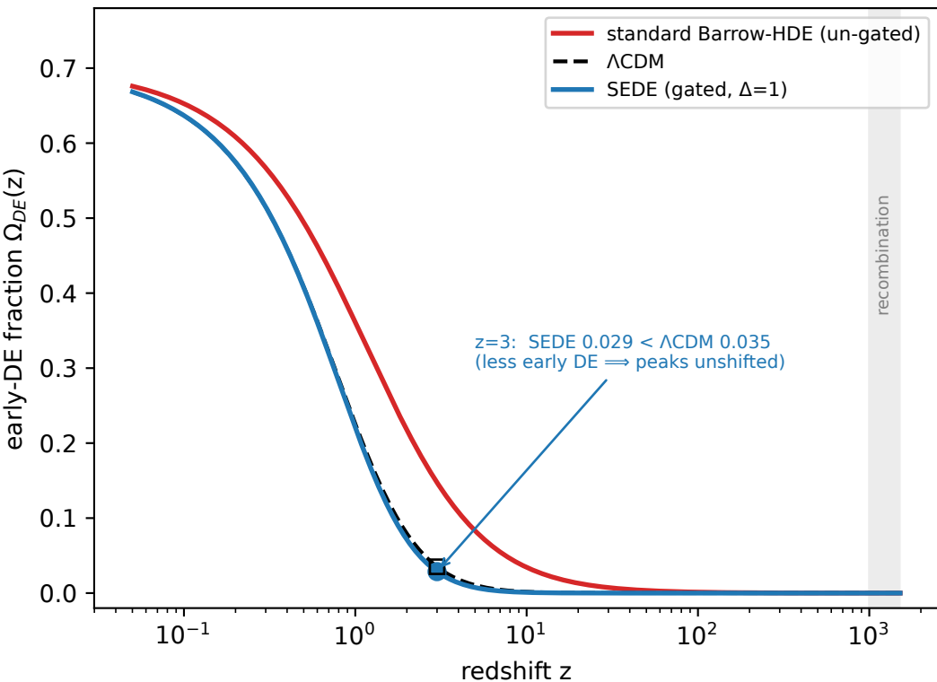
SEDE carries less early dark energy than \Lambda CDM (the gate suppresses it; HDE does not)
