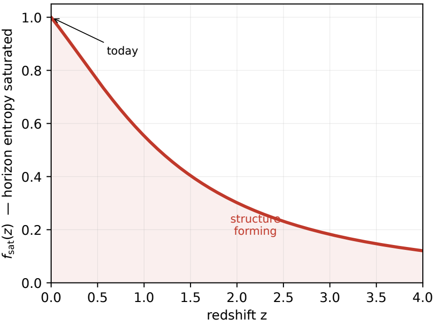
Dark energy switches on with structure
