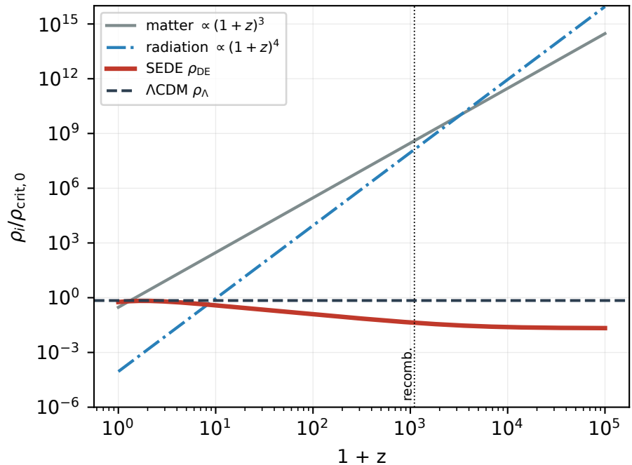
DE is negligible at high z (CMB/BBN-safe)
