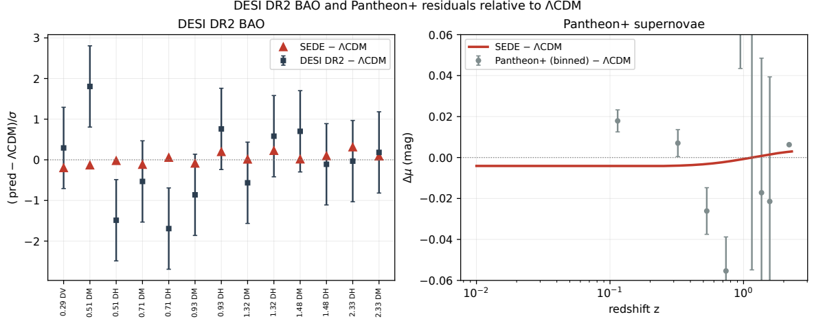
Figure 3. Matched residual comparison (relative to \Lambda CDM). Left: DESI DR2 BAO residuals relative to the \Lambda CDM best fit, in units of \sigma — the data (slate) with the SEDE prediction (red); SEDE is consistent with the measurements and sits between \Lambda CDM and the points that pull away from it. Right: Pantheon+ supernova residuals (binned) versus \Lambda CDM, with the SEDE shape overplotted. SEDE and \Lambda CDM are close at present precision; the preference is carried by the CMB-distance and H_0 channels (§5.4), not by the BAO/SN data shown here.
