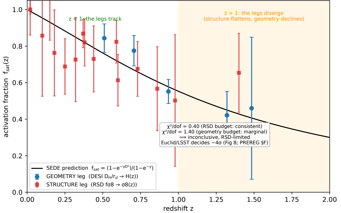
E1 — the structure-sourcing mechanism on CURRENT data SEDE's founding claim: the two legs should coincide
