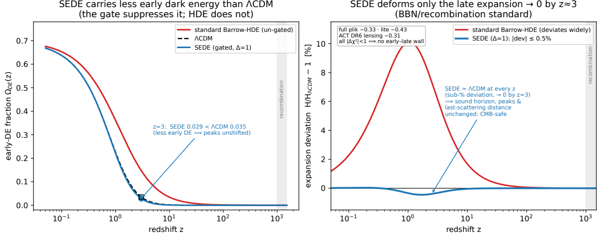
Figure 5. Why SEDE survives the CMB where standard holographic dark energy does not — the physical content of the full-CMB result (full non-lite plik \Delta\chi^2 = -0.33 , plik_{\text{lite}} - 0.43 , ACT DR6 lensing -0.31 ; all |\Delta\chi^2| < 1 ). Left: the early-dark-energy fraction \Omega_{DE}(z) . SEDE’s structure gate ( f_{\text{sat}} \rightarrow 0 at high z ) holds it below \Lambda CDM ( \Omega_{DE}(z=3) = 0.029 < 0.035 at \Omega_m = 0.30 ), whereas un-gated standard Barrow-HDE carries substantially more early DE — the runaway that drives the early–late tension of refs. [[38]]. Right: the fractional expansion deviation H/H_{\Lambda\text{CDM}} - 1 . SEDE’s deviation is sub-percent and confined to z \lesssim 3 , decaying to zero through BBN and recombination, so the sound horizon, the acoustic-peak positions, and the distance to last scattering are all essentially unchanged; standard Barrow-HDE deviates over a far wider range. SEDE has less early dark energy than \Lambda CDM, not more — hence no early–late wall.
