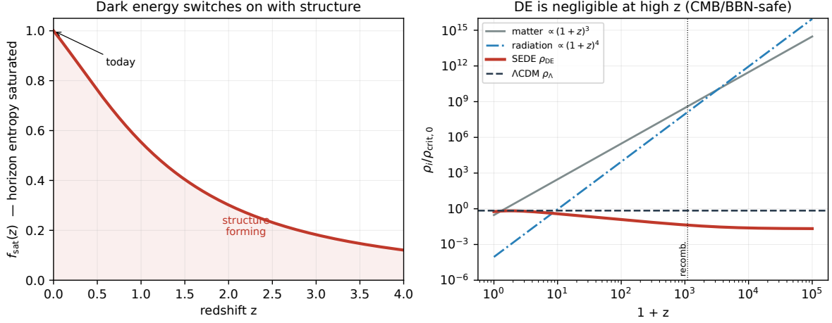
Figure 1. The mechanism. Left: the effective activation fraction (structure-growth gate) f_{\text{sat}}(z) rises toward 1 today as structure forms, activating the dark-energy gate — the effective running term \Lambda_{\text{eff}} = 3\Omega_{\text{DE}0} H H_0 f_{\text{sat}} fades in (computed from the model’s self-consistent linear growth factor D(z) , §2). Right: the cosmic density inventory; SEDE’s \rho_{\text{DE}} is orders of magnitude below matter and radiation at high z and falls below \Lambda\text{CDM} ’s constant \rho_{\Lambda} , so the early universe (BBN, recombination) is standard — the deformation acts only on the late-time dark-energy fluid.
