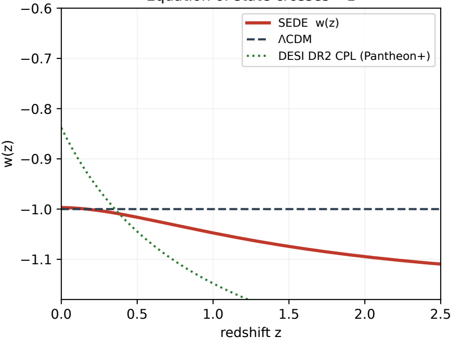
Equation of state crosses -1
