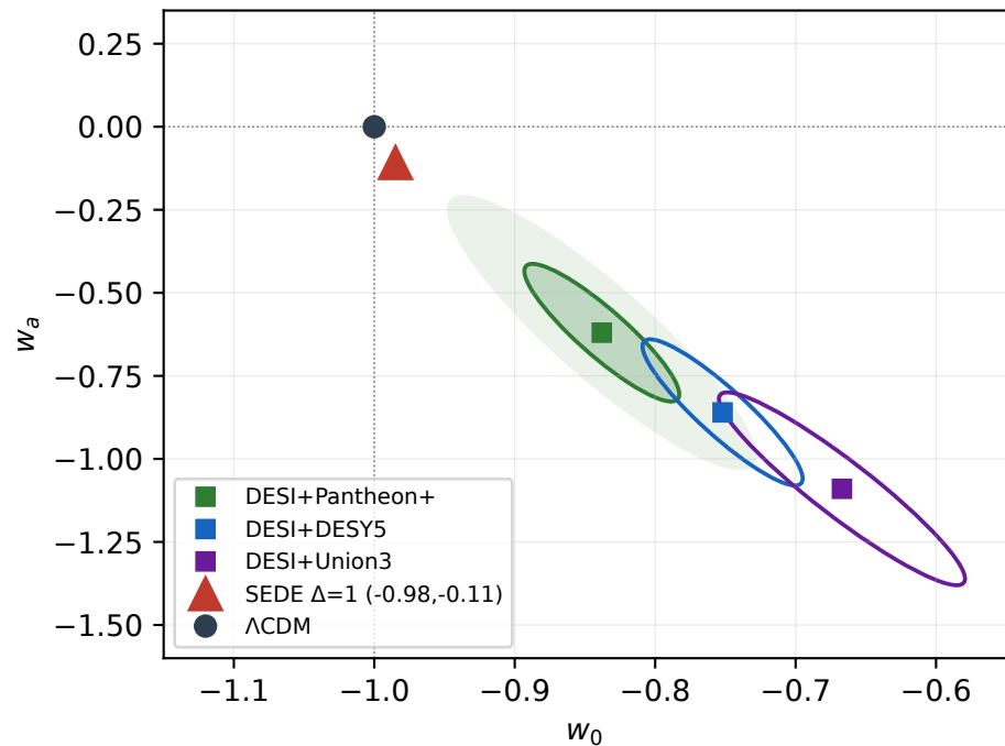
In DESI's evolving-DE quadrant (official DR2 chains)
