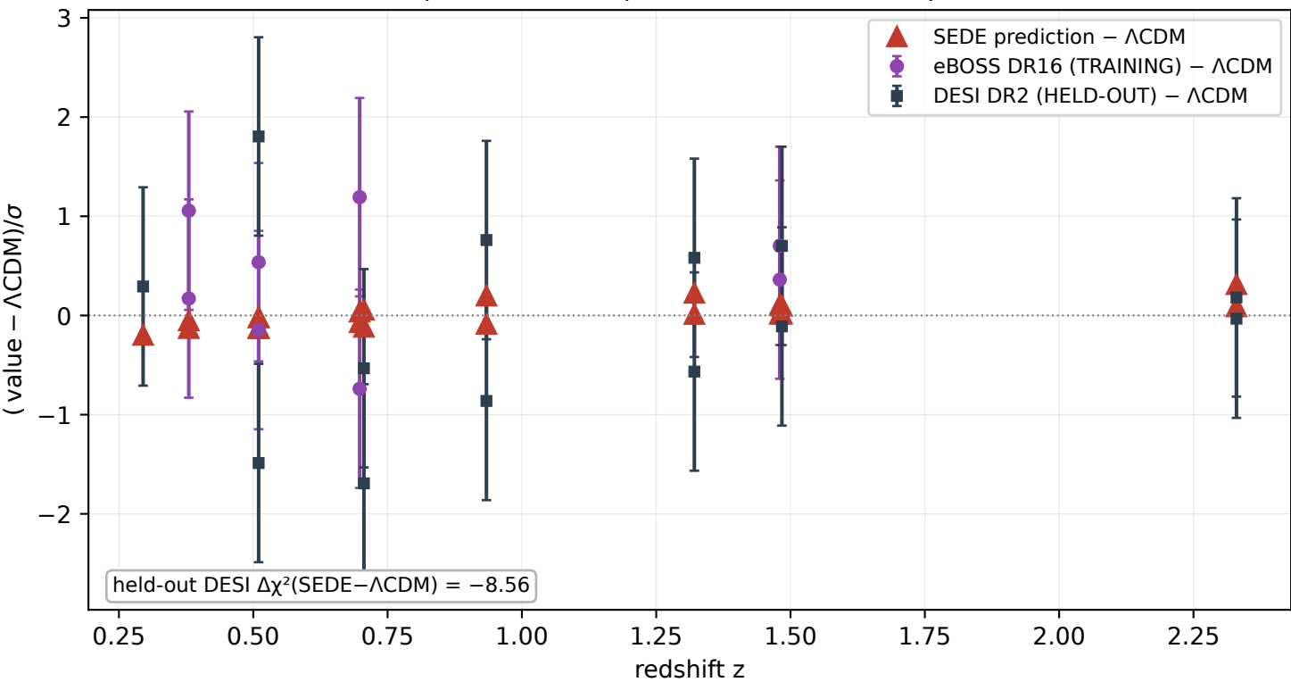
Out-of-sample: trained on pre-DESI eBOSS, SEDE predicts DESI
