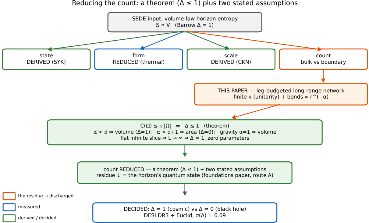
FIG. 1. The reduction. SEDE's one input — volume-law horizon entropy — decomposes into state , form , scale , and count (the foundations paper); the first three reduce to established physics, and the count is the irreducible residue. Modelling the horizon degrees of freedom as a leg-budgeted long-range network reduces it: C(\Omega) \leq \kappa \cdot |\Omega| makes \Delta \leq 1 a theorem (§II B), \alpha < d puts gravity on the volume branch (§II C–§IV), and \Delta = 1 is the L \rightarrow \infty endpoint of the flat infinite slice — a cutoff choice, not a derivation (§V). What survives is the horizon's quantum state (route A of the foundations paper) and that endpoint identification, decided — with the black-hole \Delta = 0 — by DESI DR3 + Euclid.
