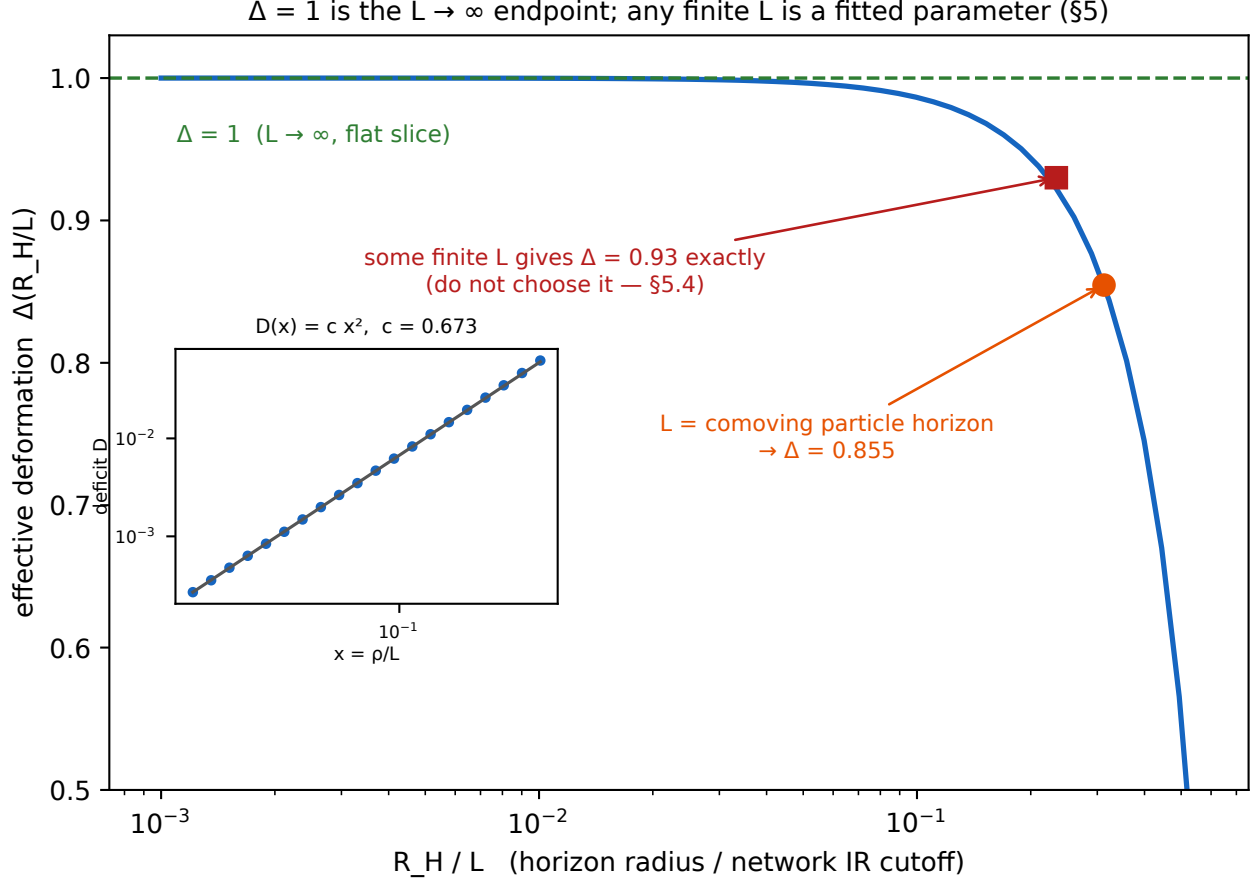
FIG. 4. \Delta = 1 and the infrared cutoff (§V). The effective deformation \Delta(R_H/L) rises to 1 as the network cutoff L \rightarrow \infty . Nothing in the model fixes L , so any finite value is a fitted dark-sector parameter — and choosing one is choosing the answer: L = the comoving particle horizon returns \Delta = 0.855 , and some L reproduces the foundations paper’s profile value 0.93 exactly (§V D cautions against both). Identifying the flat, infinite spatial slice with the network cutoff takes L \rightarrow \infty and \Delta = 1 — the endpoint choice of §V C, which eliminates the parameter without deriving the value. Inset: the exact deficit law D(x) = c \cdot x^2 at \alpha = 1 (Newton kernel), c = 0.673 .
