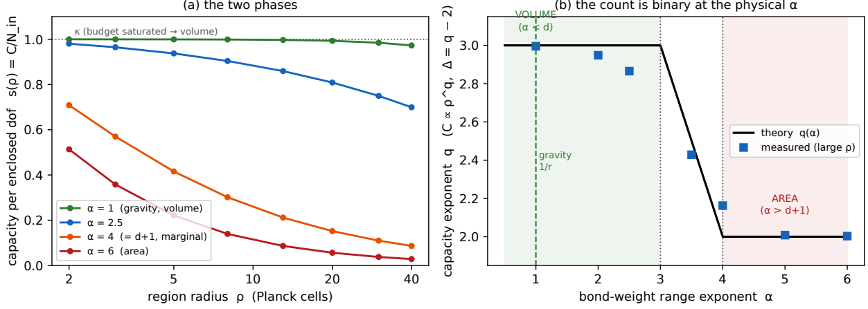
FIG. 2. The binary count (§II C–2.4). (a) Capacity per enclosed degree of freedom s(\rho) = C/N_{in} : at \alpha = 1 (gravity) it saturates the leg budget \kappa (the volume law); at \alpha = 6 it falls as 1/\rho (the area law). (b) The capacity exponent q (with \Delta = q - 2 ) versus the bond-range \alpha : q = 3 (volume) for every \alpha < d and q = 2 (area) for \alpha > d + 1 , interpolating only in the unphysical window d < \alpha < d + 1 (the marginal \alpha = d + 1 = 4 point carries a logarithm, so its finite- \rho value sits just above 2). Gravity’s 1/r reach ( \alpha = 1 ) lies deep in the volume basin; no gravitational coupling yields an intermediate \Delta .
