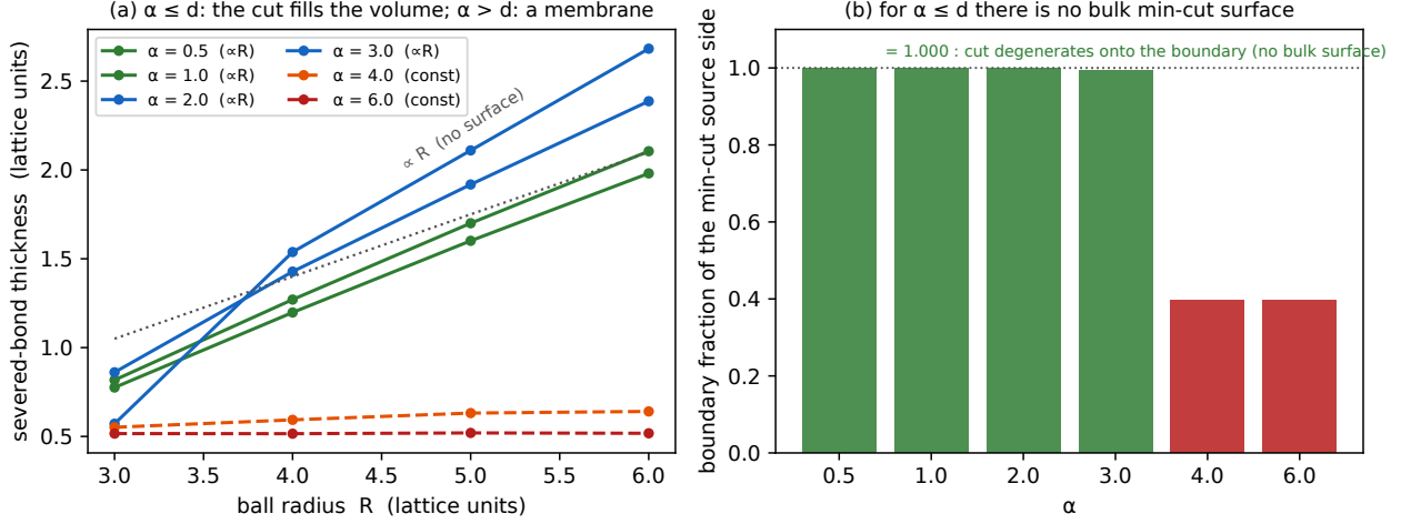
FIG. 3. No minimum-cut surface for a long-range horizon (§II E). (a) The thickness of the severed-bond set grows \propto R for \alpha \leq d (the cut fills the volume — there is no surface) and is R -independent for \alpha > d (a one-cell membrane). (b) The boundary fraction of the minimum cut’s source side is 1.000 for \alpha \leq d (the cut degenerates onto the boundary shell) and \approx 0.40 for \alpha > d (a genuine bulk membrane). With no min-cut surface there is no height field, no roughness exponent, and no roughening — so \Delta is a count, not a Hausdorff dimension.
